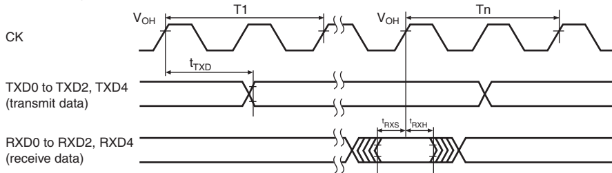
Figure 33.46 SCI Input/Output Timing
