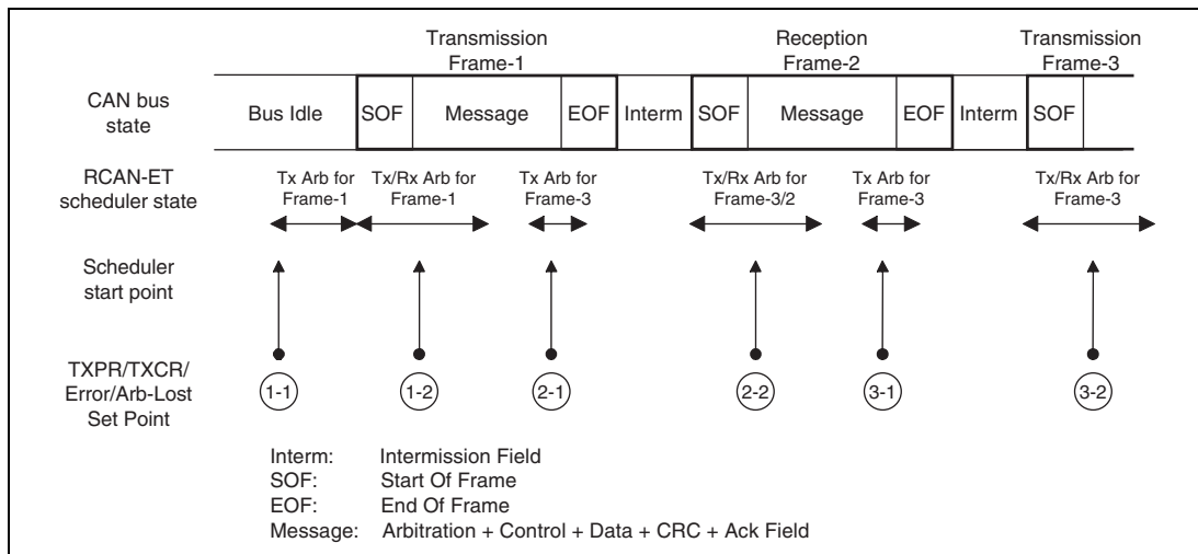
Figure 21.11 Internal Arbitration for Transmission
