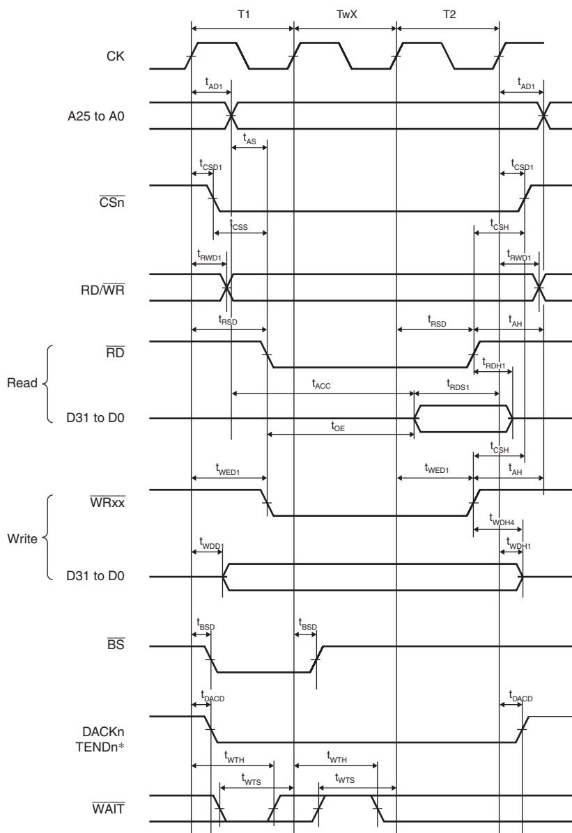
Figure 33.12 Basic Bus Timing for Normal Space (One External Wait Cycle)
