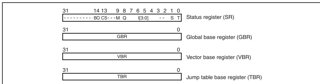
Figure 2.3 Control Registers
