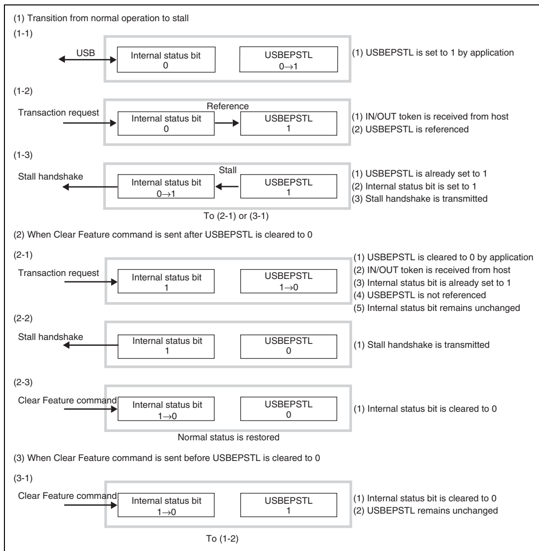
Figure 24.14 Forcible Stall by Application
