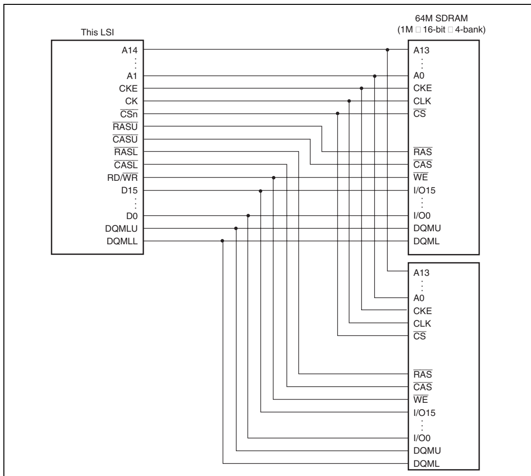
Figure 9.16 Example of 16-Bit Data Width SDRAM Connection ( \overline{RASU} and \overline{CASU} are Used)
