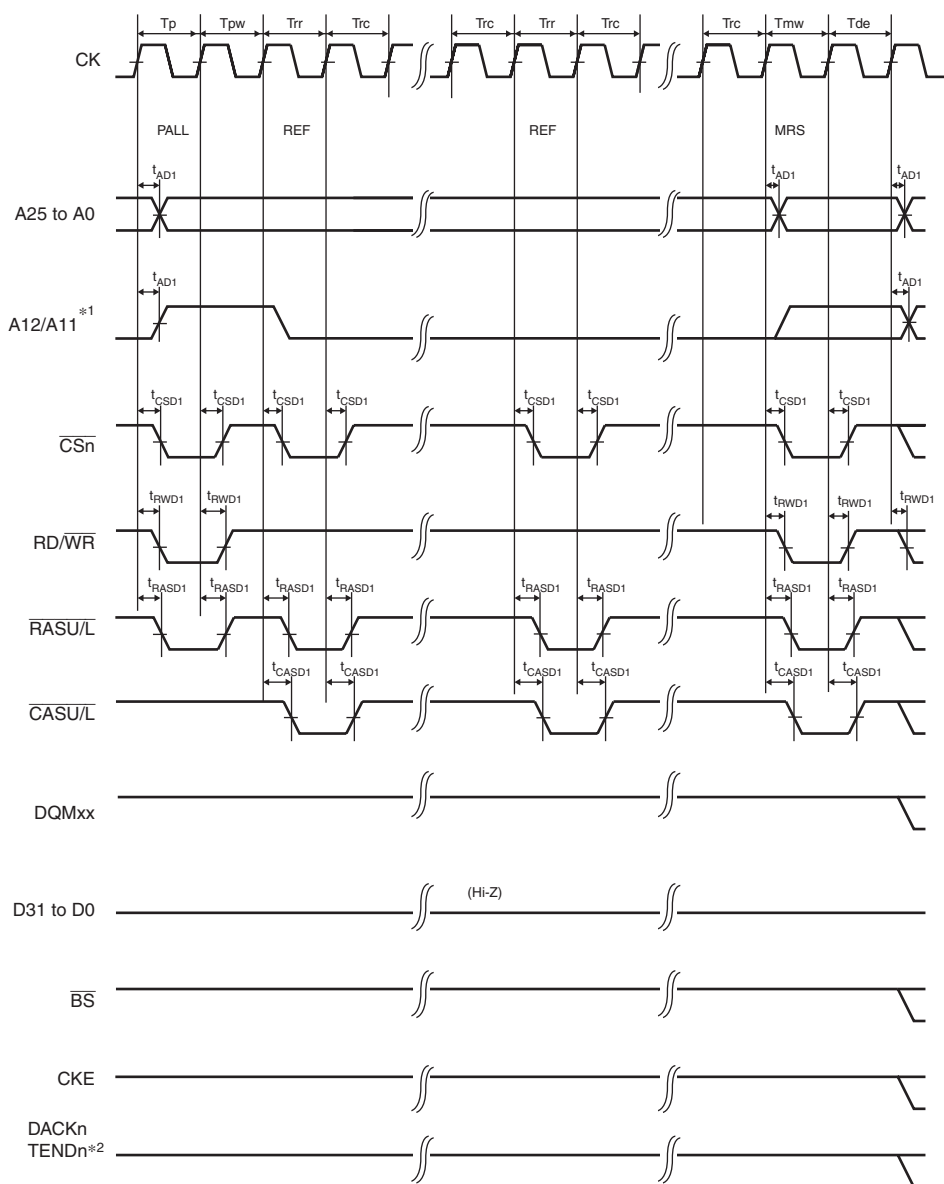
Figure 33.34 Synchronous DRAM Mode Register Write Timing (WTRP = 1 Cycle)
