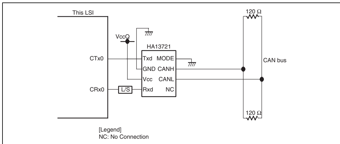
Figure 21.16 High-Speed CAN Interface Using HA13721
