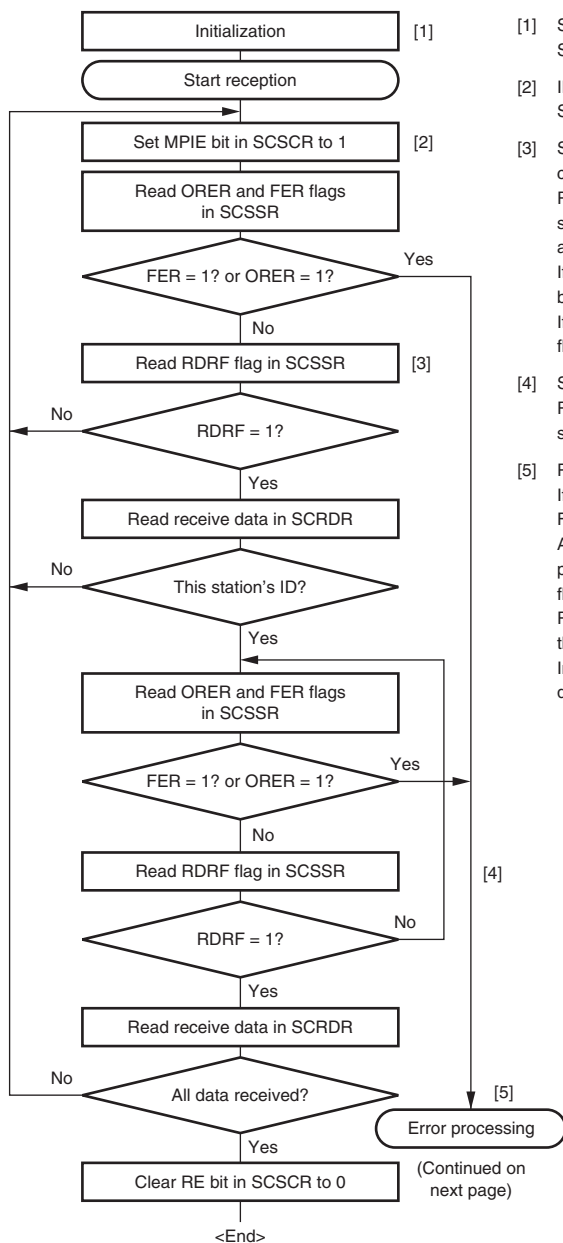
Figure 16.18 Sample Multiprocessor Serial Reception Flowchart (1)
