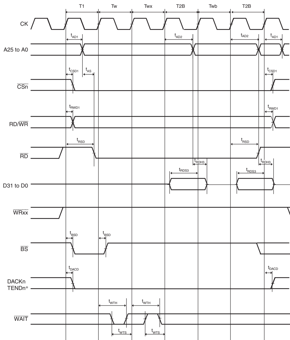
Figure 33.17 Burst ROM Read Cycle (One Software Wait Cycle, One Asynchronous External Burst Wait Cycle, Two-Cycle Burst)
