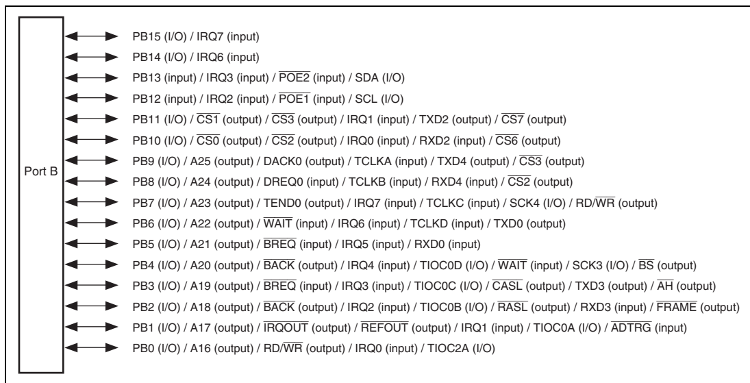
Figure 23.2 Port B
