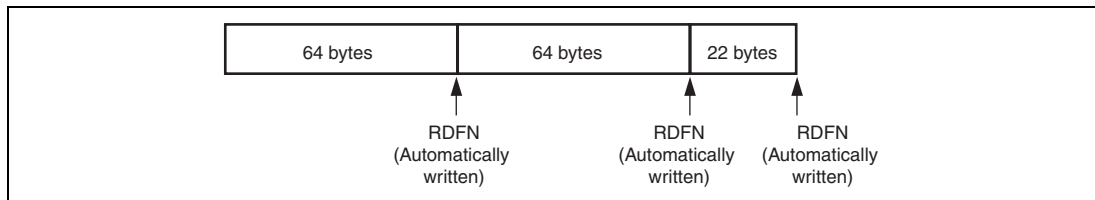
Figure 24.16 EP1/EP4 RDFN (EP1RDFN, EP4RDFN) Operation
