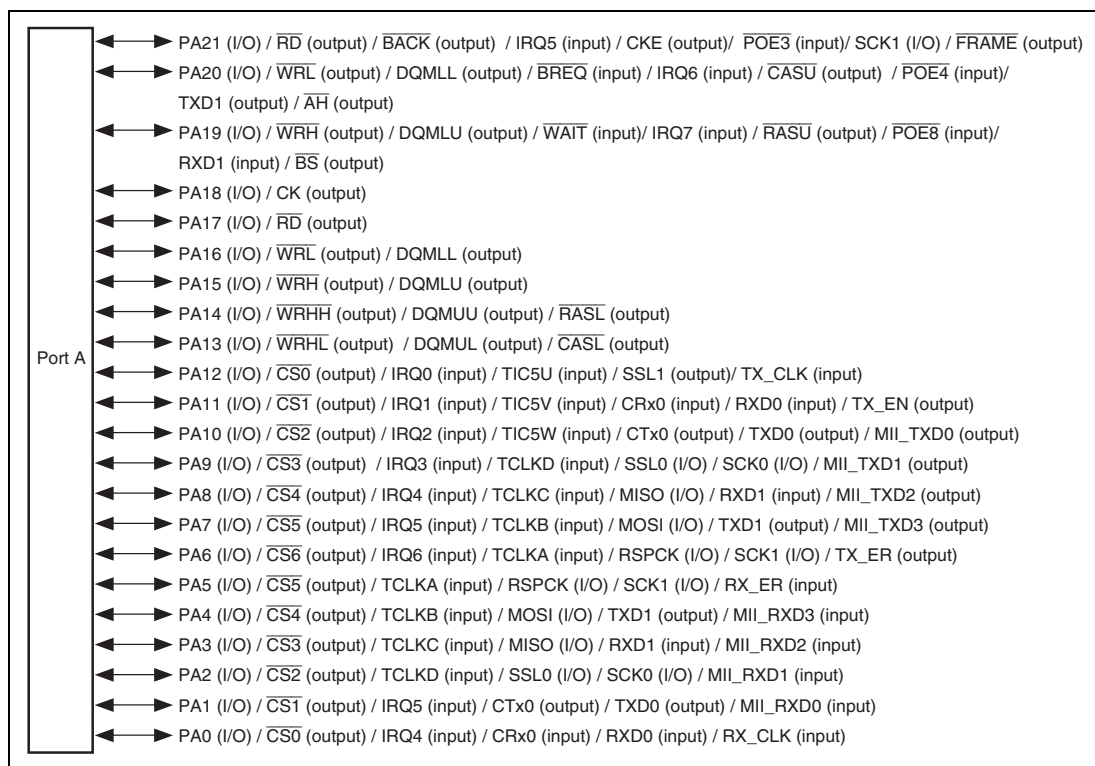
Figure 23.1 Port A
