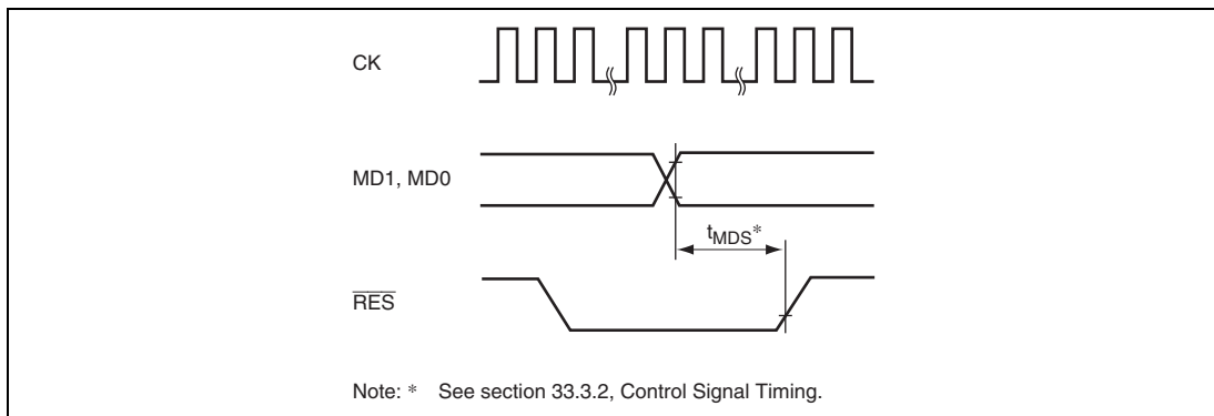
Figure 3.4 Reset Input Timing when Changing Operating Mode
