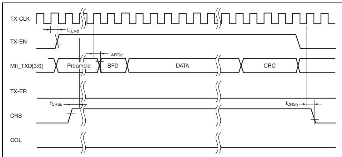
Figure 33.58 MII Transmission Timing (during Normal Operation)
