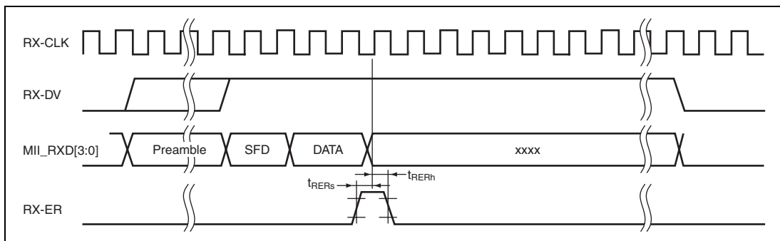
Figure 33.61 MII Reception Timing (in the Event of an Error)
