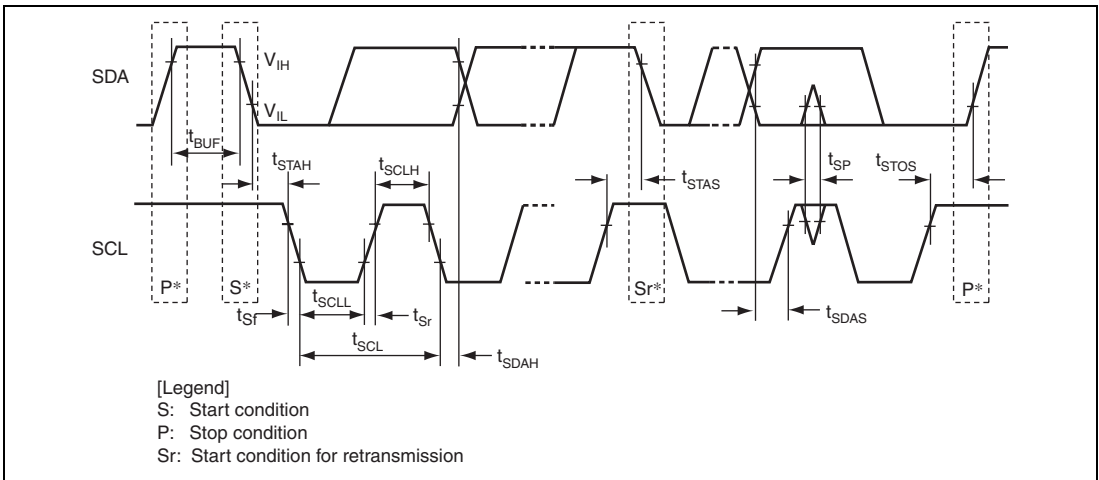
Figure 33.55 I 2 C Bus Interface 3 Input/Output Timing
