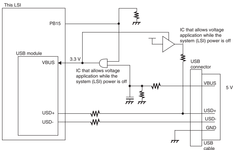
Figure 24.28 Example of USB Function Module External Circuitry
