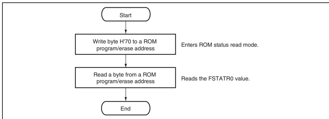
Figure 27.27 Procedure for Checking Status Register 0
