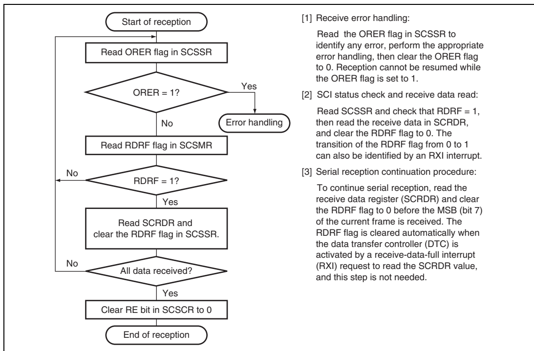
Figure 16.12 Sample Flowchart for Receiving Serial Data (1)
