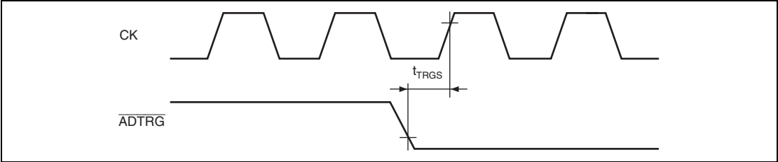
Figure 33.56 A/D Converter External Trigger Input Timing
