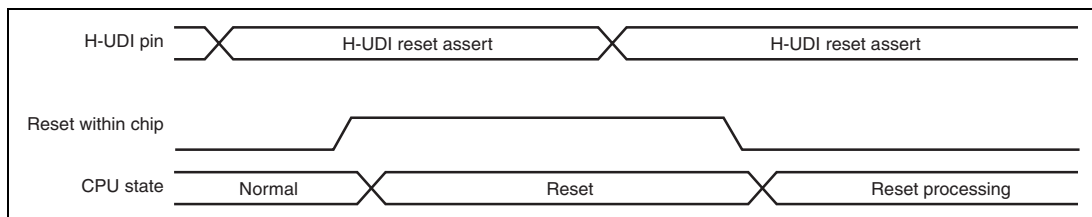
Figure 31.4 H-UDI Reset
