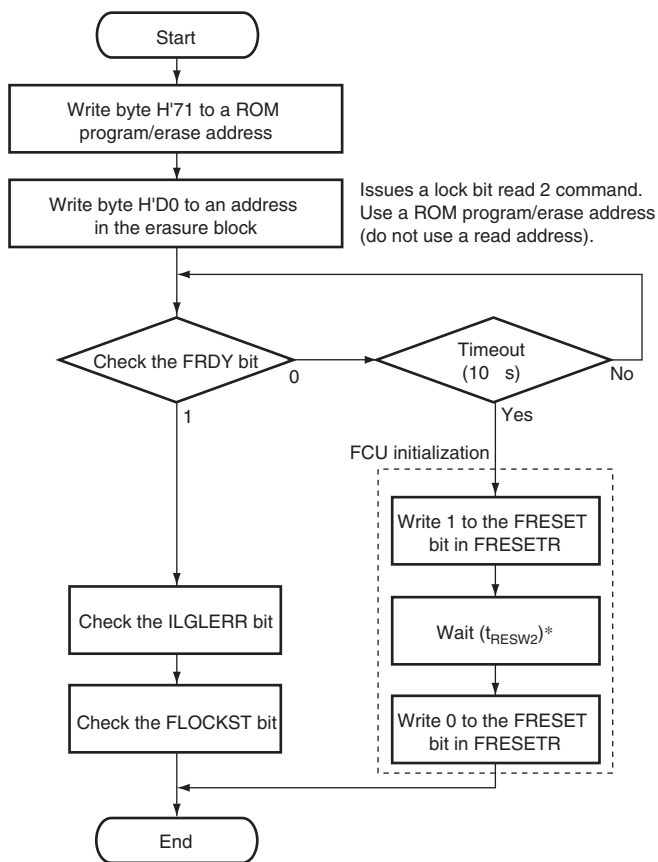
Figure 27.29 Procedure for Reading Lock Bit in Register Read Mode
