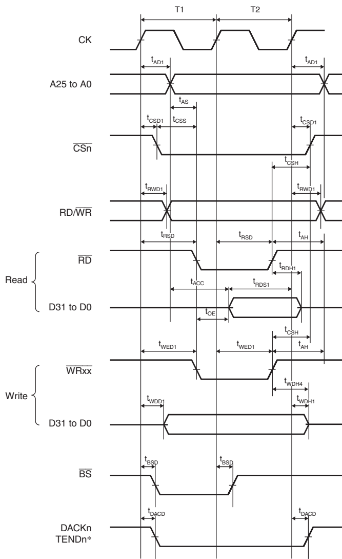
Figure 33.10 Basic Bus Timing for Normal Space (No Wait)
