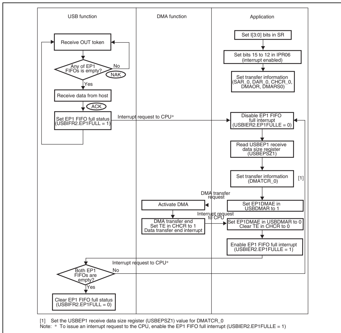
Figure 24.18 Example of DMA Transfer (Channel 0) for Bulk-OUT Transfer (EP1) (When Receive Data Size Cannot be Determined Before Receiving OUT Token)
