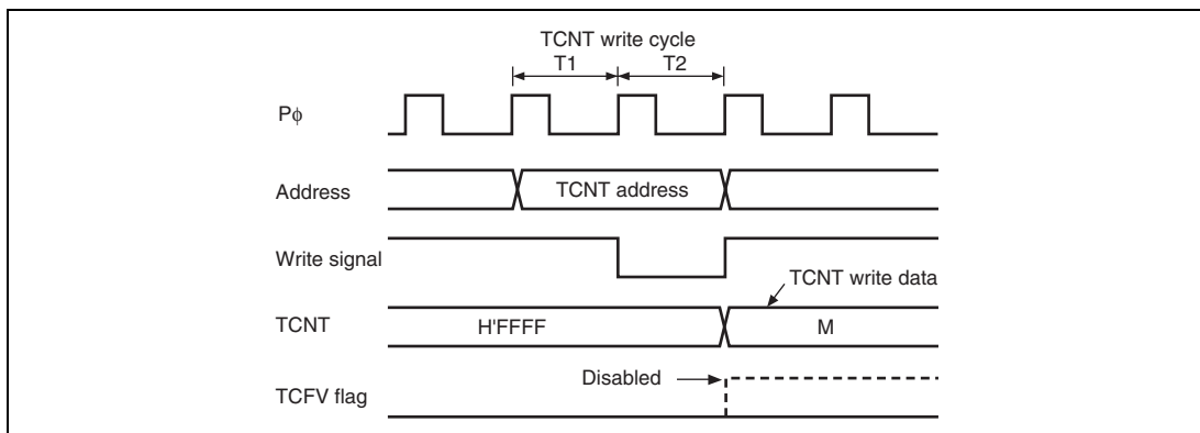
Figure 11.136 Contention between TCNT Write and Overflow
