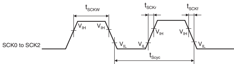
Figure 33.45 Input Clock Timing
