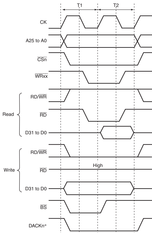
Figure 9.37 Basic Access Timing for SRAM with Byte Selection (BAS = 0)
