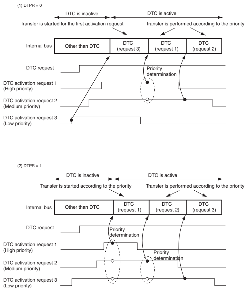
Figure 8.17 Example of DTC Activation According to Priority
