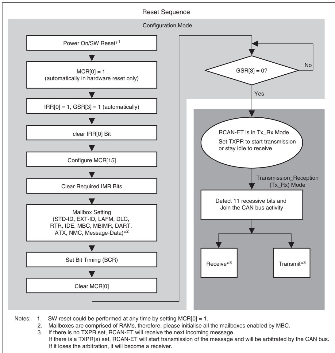
Figure 21.8 Reset Sequence
