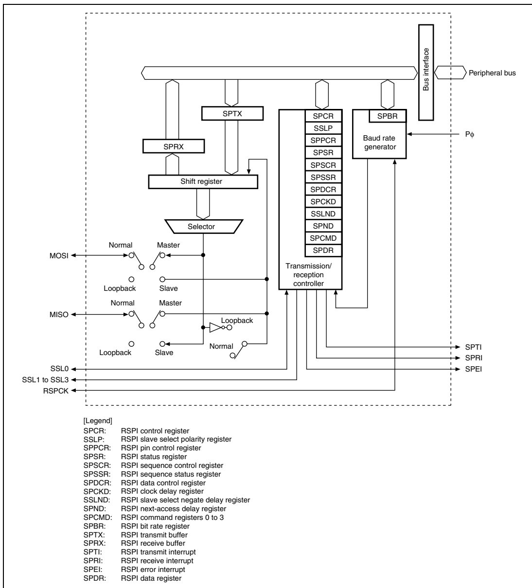
Figure 18.1 Block Diagram of RSPI
