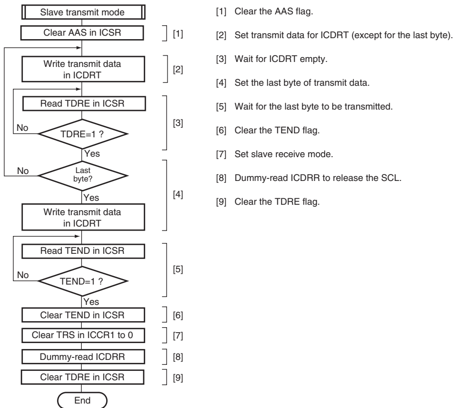
Figure 19.21 Sample Flowchart for Slave Transmit Mode
