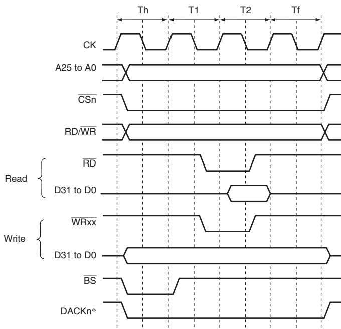
Figure 9.10 \overline{\text{CSn}} Assert Period Expansion
