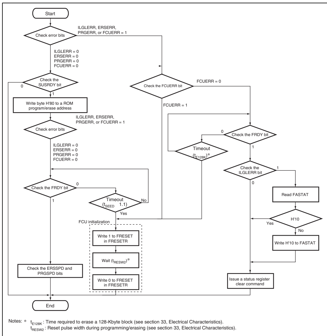
Figure 27.24 Procedure for Programming/Erase Suspension
