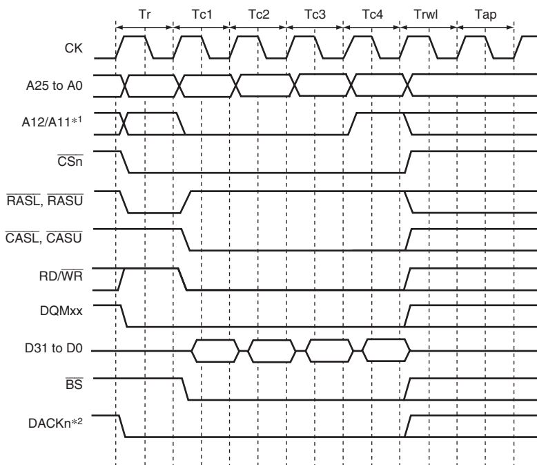
Figure 9.21 Basic Timing for Burst Write (Auto-Precharge)
