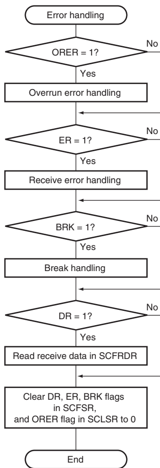
Figure 17.7 Sample Flowchart for Receiving Serial Data (cont)
