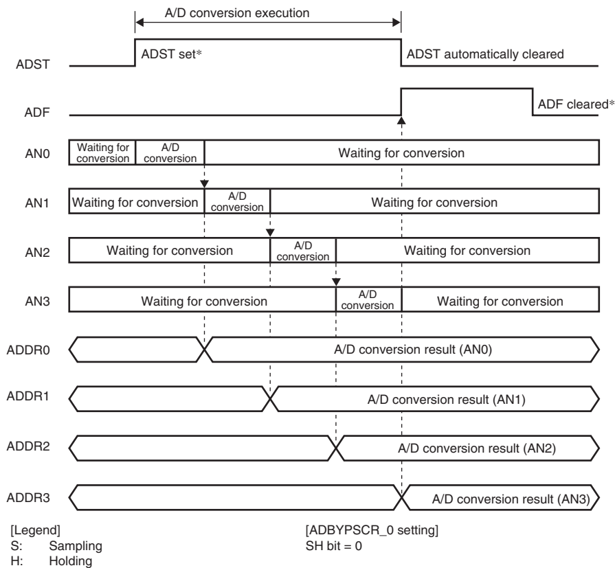
Figure 20.3 Example 2 of A/D_0 Converter Operation (Single-Cycle Scan Mode and Sample-and-Hold Circuit Disabled)
