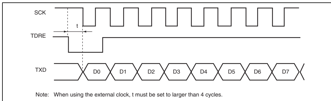
Figure 16.22 Example of Clock Synchronous Transfer Using DTC
