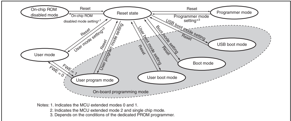
Figure 27.4 ROM-Related Mode Transition
