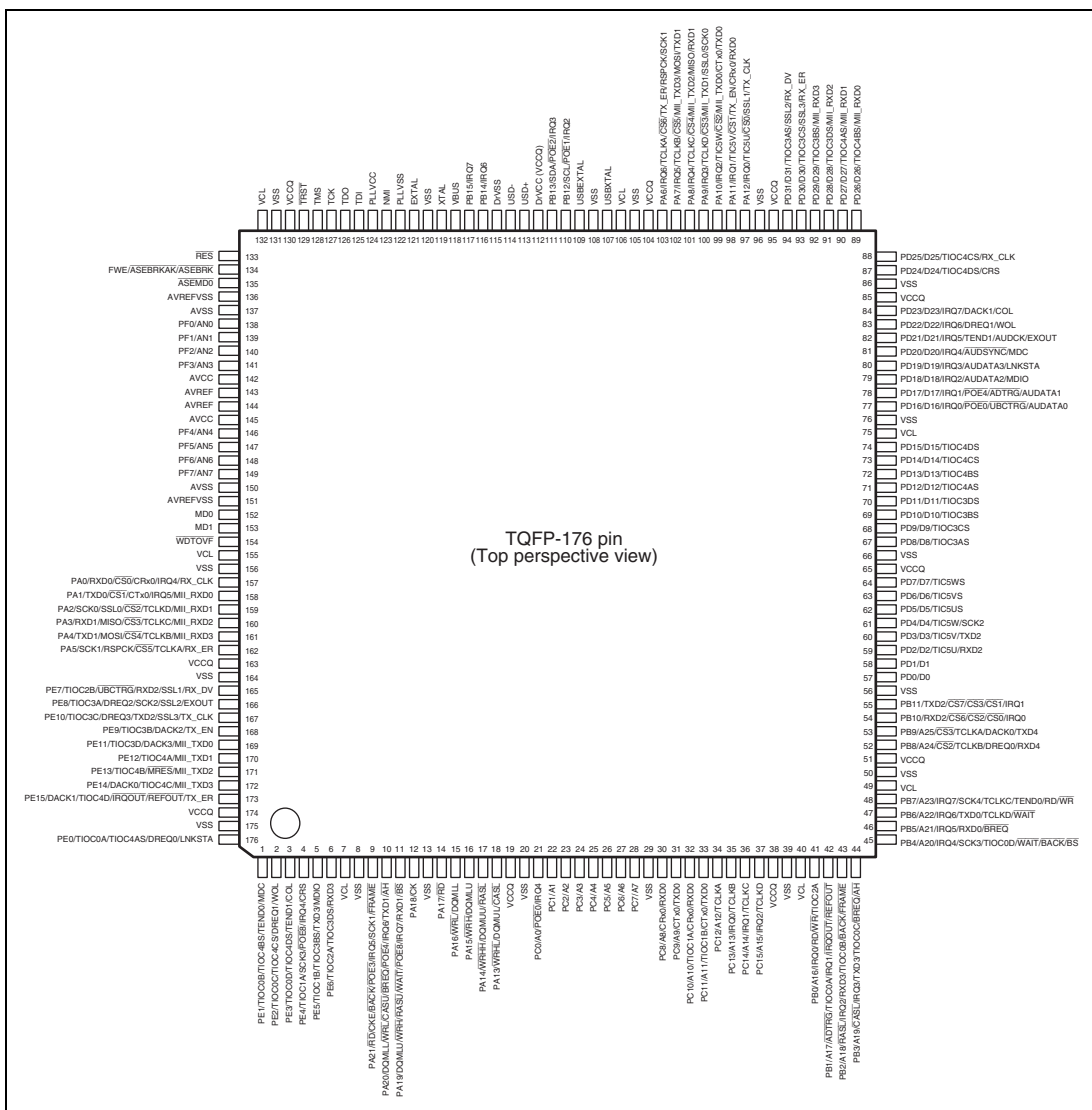
Figure 1.2 Pin Assignment (1)
