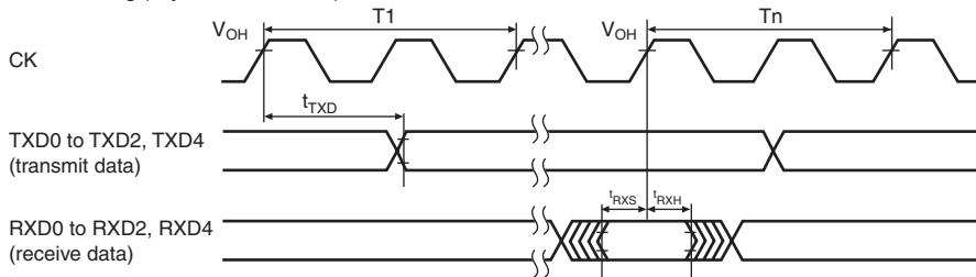
Figure 33.46 SCI Input/Output Timing
