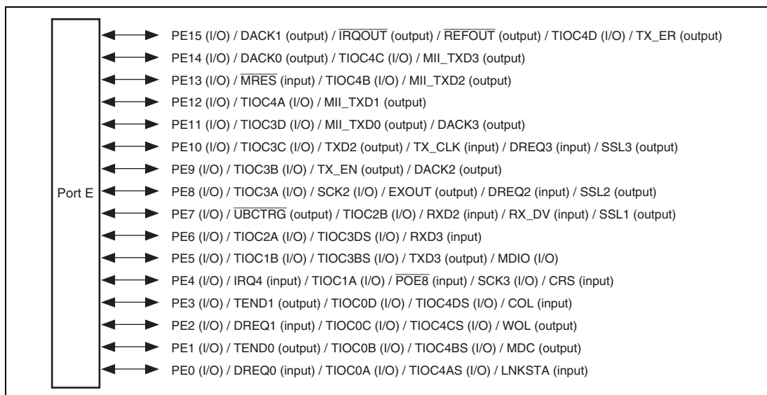
Figure 23.5 Port E
