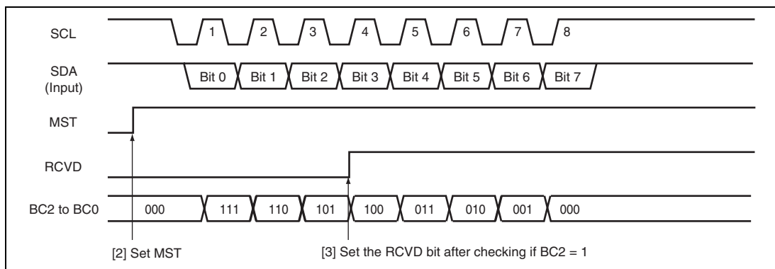
Figure 19.16 Operation Timing For Receiving One Byte (MST = 1)
