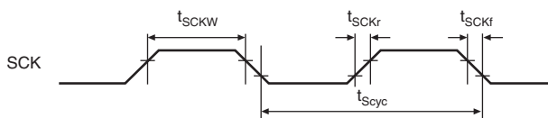
Figure 33.47 SCK Input Clock Timing
