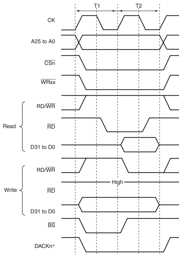
Figure 9.38 Basic Access Timing for SRAM with Byte Selection (BAS = 1)
