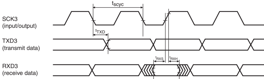
SCI I/O timing (clocked synchronous mode)
