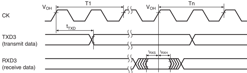
SCI I/O timing (asynchronous mode)
