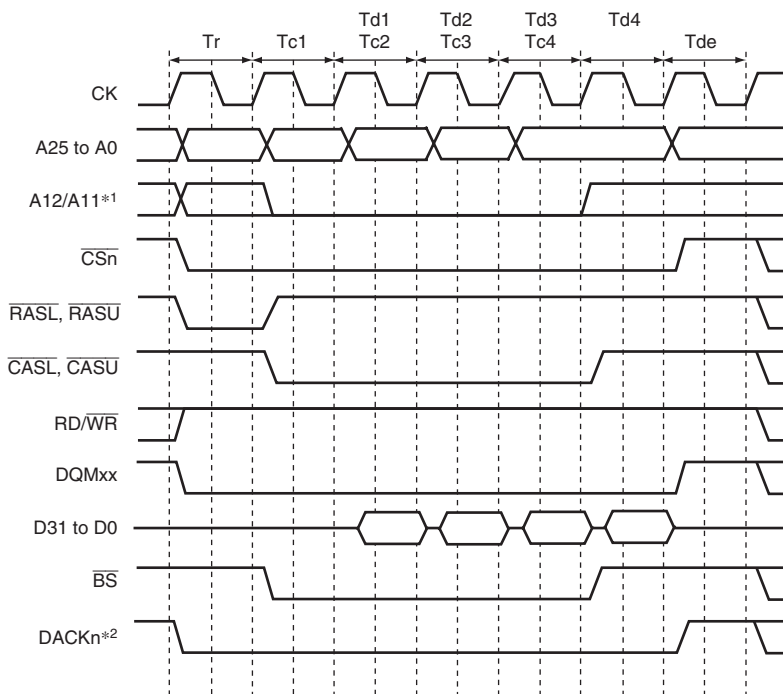
Figure 9.23 Burst Read Timing (Bank Active, Different Bank, CAS Latency 1)
