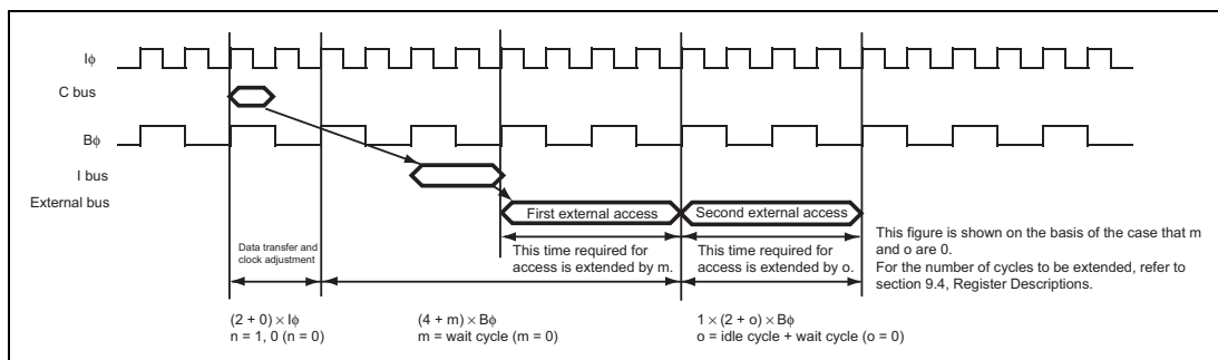
Figure 9.48 Timing of Write Access to Data Beyond External Bus Width When I\phi:B\phi = 2:1
