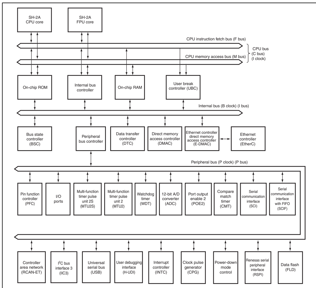
Figure 1.1 Block Diagram
