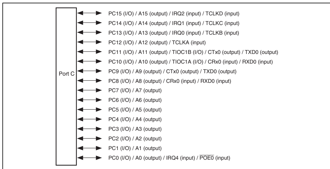
Figure 23.3 Port C
