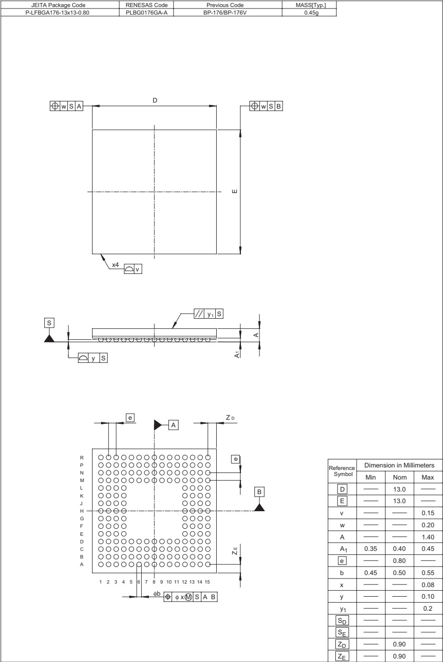
Figure C.3 Package Dimensions (3)
