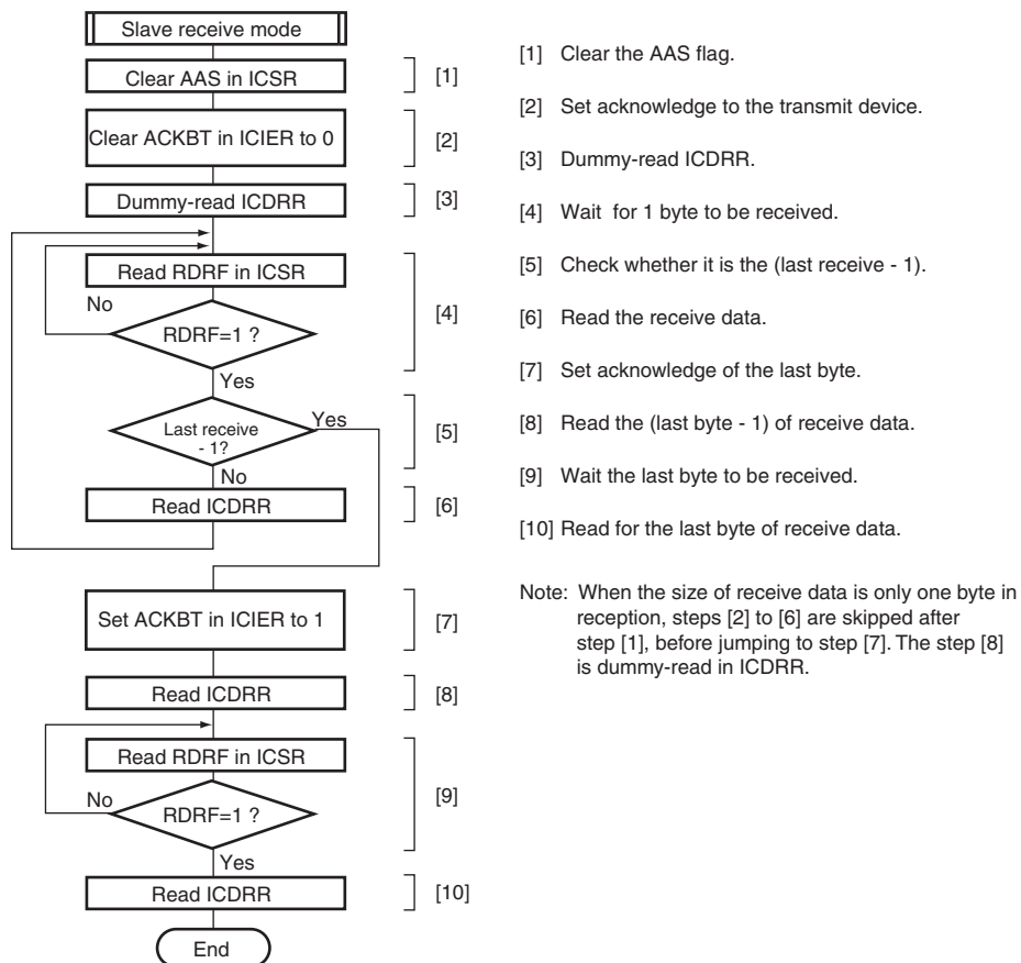
Figure 19.22 Sample Flowchart for Slave Receive Mode
