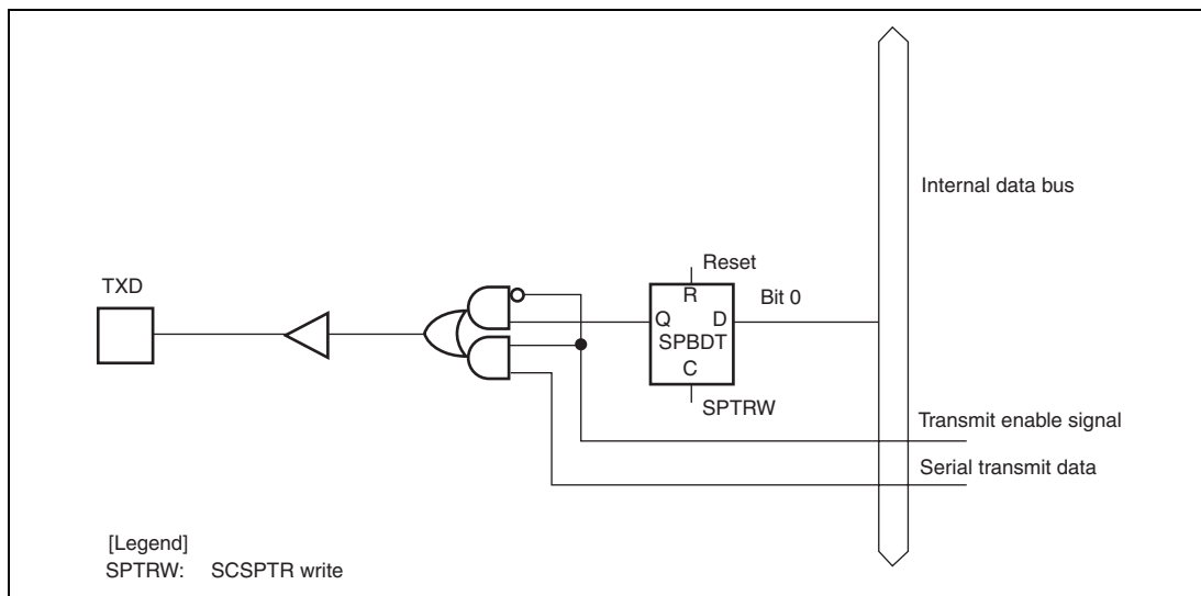
Figure 16.20 SPBDT Bit and TXD Pin
