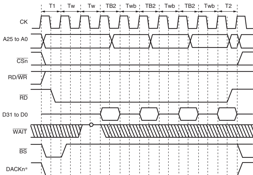
Figure 9.36 Burst ROM Access Timing (Clock Asynchronous) (Bus Width = 32 Bits, 16-Byte Transfer (Number of Burst 4), Wait Cycles Inserted in First Access = 2, Wait Cycles Inserted in Second and Subsequent Access Cycles = 1)
