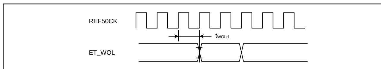
Figure 5.52 WOL Output Timing (RMI)
