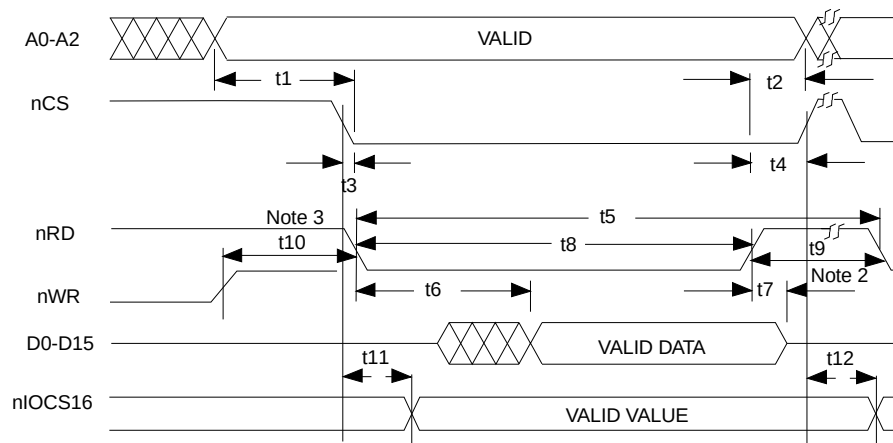
FIGURE 8-6: NON-MULTIPLEXED BUS, 80XX-LIKE CONTROL SIGNALS; READ CYCLE
