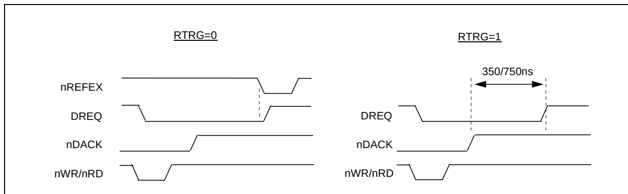
FIGURE 6-1: ILLUSTRATION OF THE EFFECT OF RTRG BIT ON DMA TIMING
