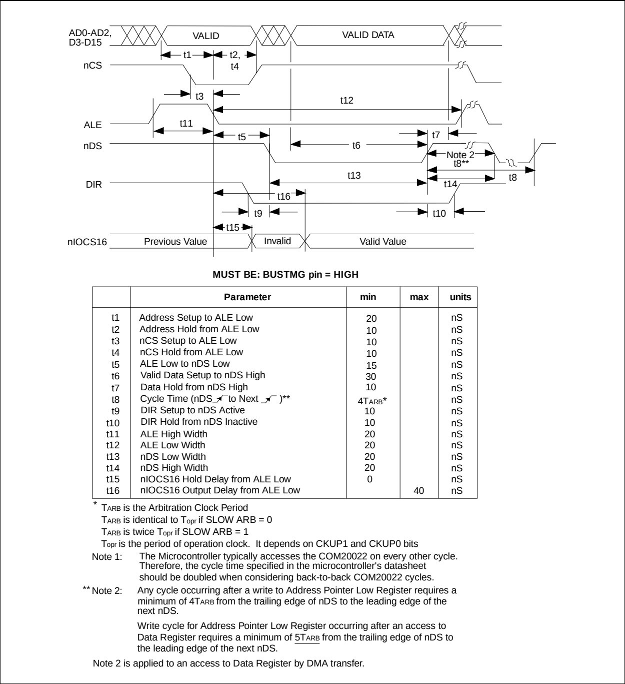
FIGURE 8-3: MULTIPLEXED BUS, 68XX-LIKE CONTROL SIGNALS WRITE CYCLE
