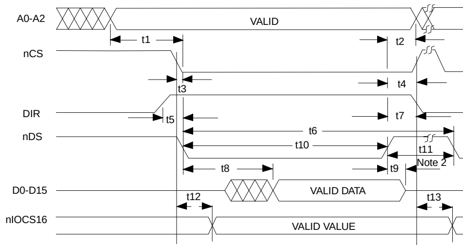
FIGURE 8-8: NON-MULTIPLEXED BUS, 68XX-LIKE CONTROL SIGNALS; READ CYCLE
