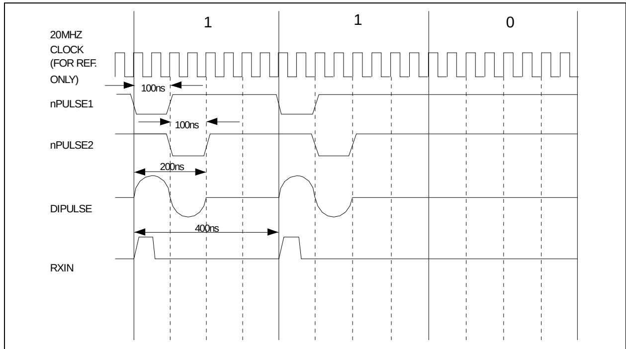
FIGURE 5-9: DIPULSE WAVEFORM FOR DATA OF 1-1-0
