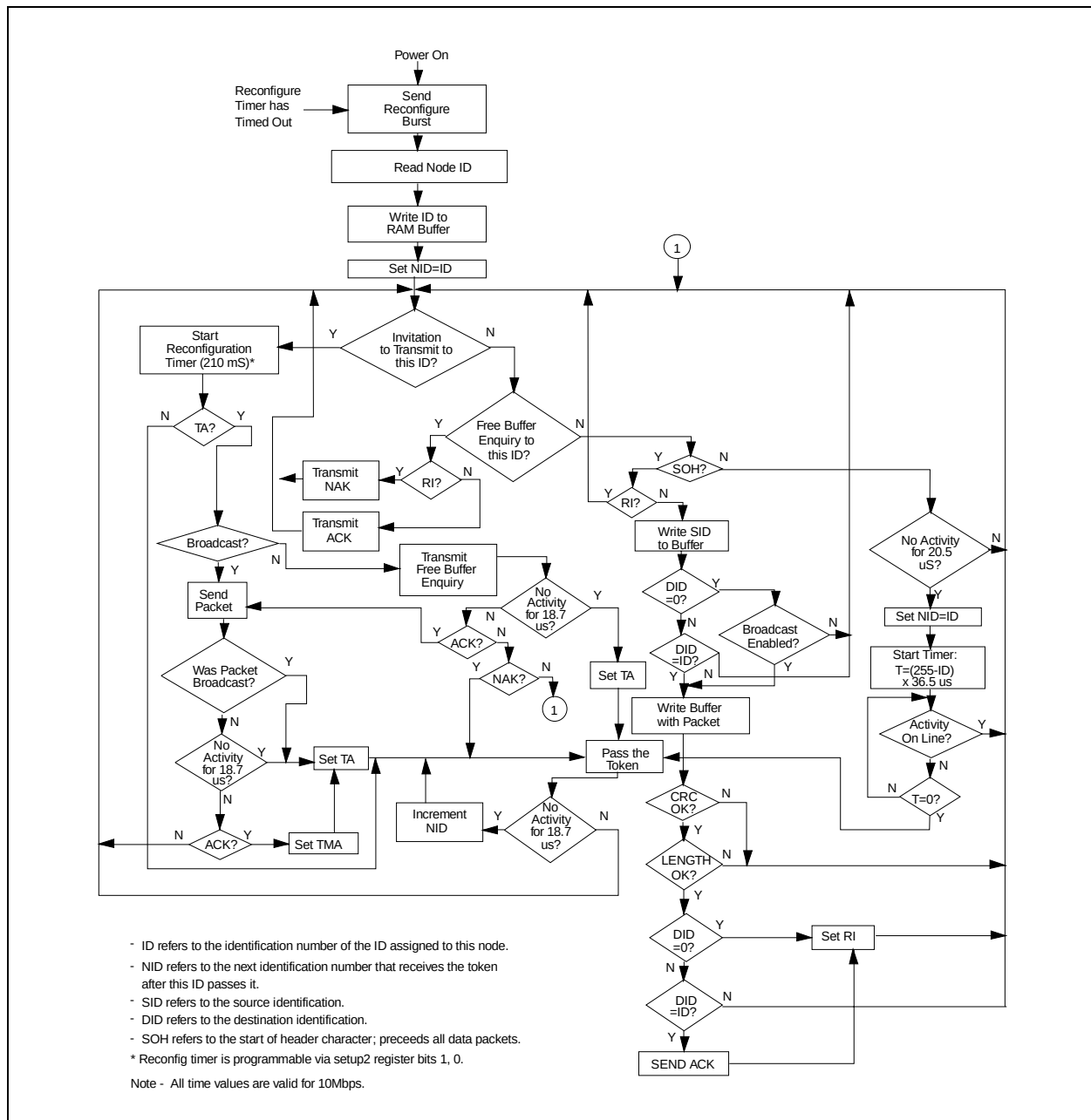
FIGURE 3-1: COM20022I OPERATION
