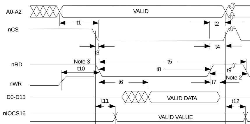
FIGURE 8-5: NON-MULTIPLEXED BUS, 80XX-LIKE CONTROL SIGNALS; READ CYCLE
