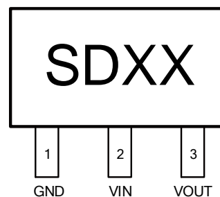
TO-92
