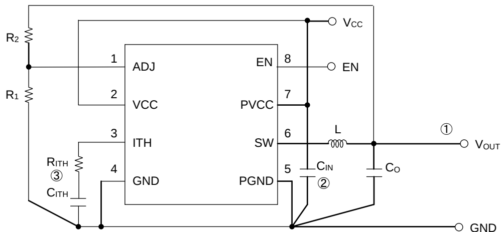
Figure 36. Layout Diagram
