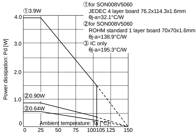
Figure 27. Thermal Derating Curve (SON008V5060)
