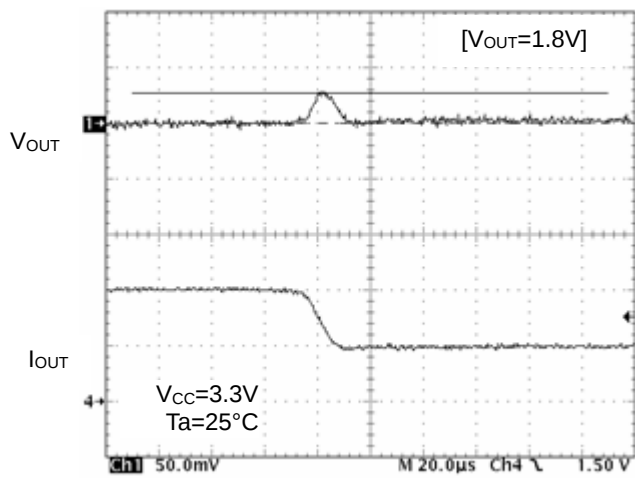
Figure 18. Transient Response (Io=2A to 1A, 10µs)
