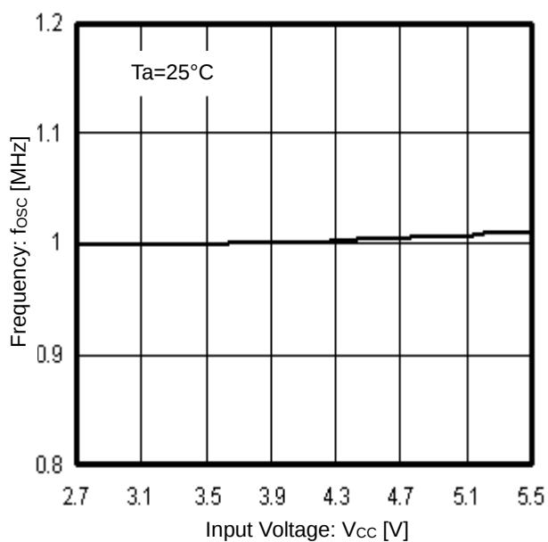
Figure 13. Frequency vs Input Voltage
