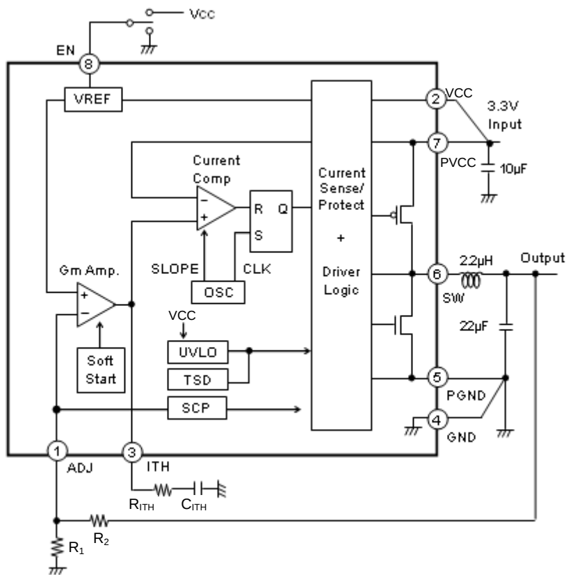
Figure 3. Block Diagram
