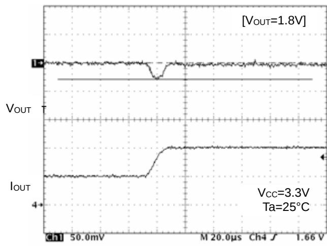
Figure 17. Transient Response (Io=1A to 2A, 10µs)
