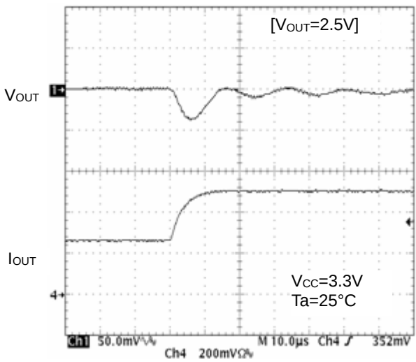
Figure 17. Transient Response (Io=250mA to 500mA, 10μs)
