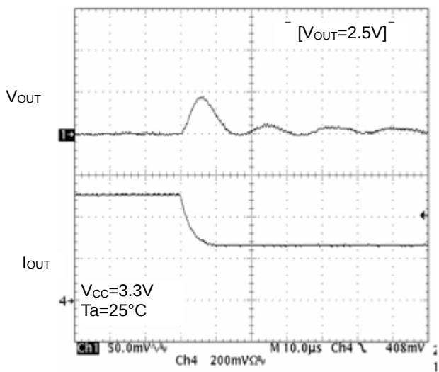
Figure 18. Transient Response (Io=500mA to 250mA, 10μs)
