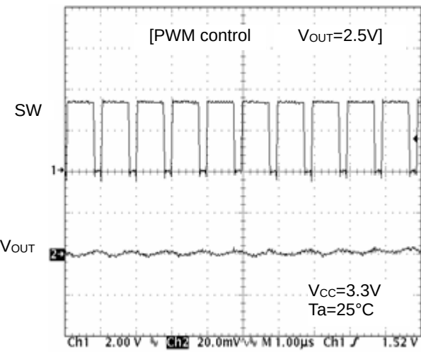
Figure 15. SW Waveform (Io=500mA)
