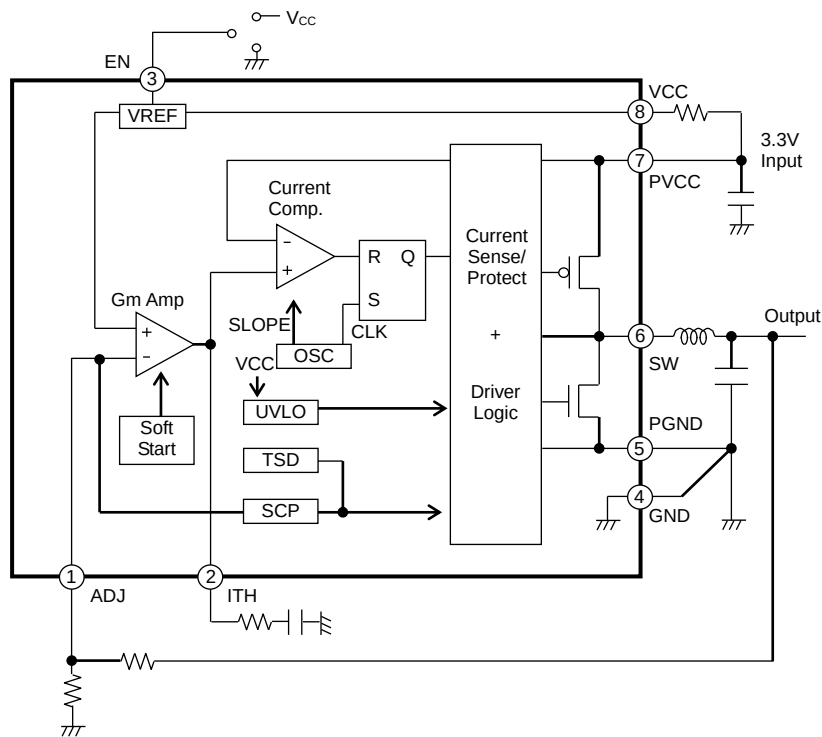
Figure 3. Block Diagram
