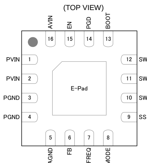
Figure 2. Pin Assignment
