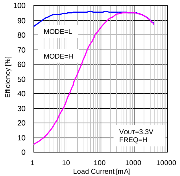
Figure 9. Efficiency vs Load Current ( V_{IN}=5V , V_{OUT}=3.3V , L=1.0\mu H , FREQ=H )
