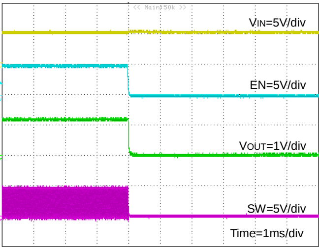
Figure 29. Power Down Waveform with EN (FREQ=H, RLOAD=0.3Ω)
