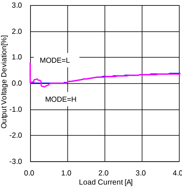
Figure 37. Load Regulation (VIN=5V, VOUT=1.2V, L=1.0μH, FREQ=H)
