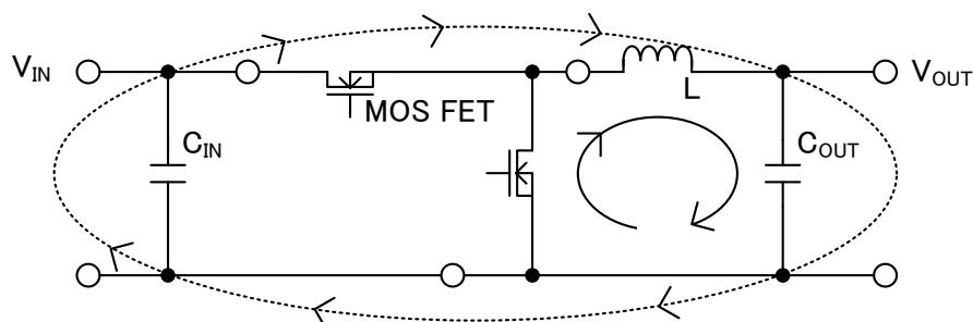
Figure 52. Current Loop of Buck Converter
