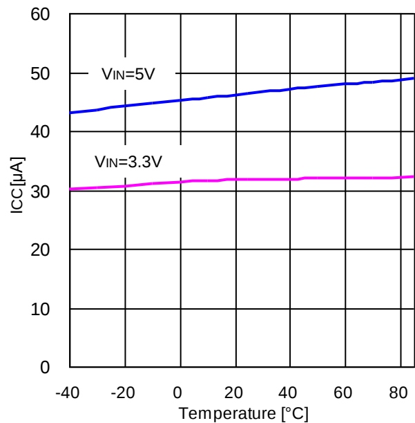
Figure 4. Operating Supply Current vs Temperature
