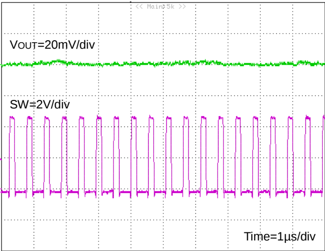
Figure 33. Switching Waveform ( V_{IN}=5\text{V} , V_{OUT}=1.2\text{V} , \text{FREQ}=\text{L} , I_{OUT}=4\text{A} )
