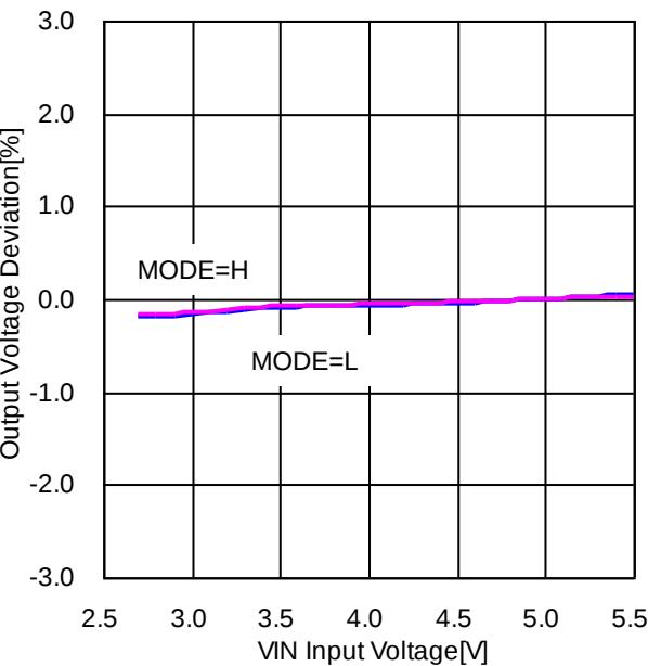
Figure 36. Line Regulation (VOUT=1.2V, L=1.0μH, FREQ=H, IOUT=4A)
