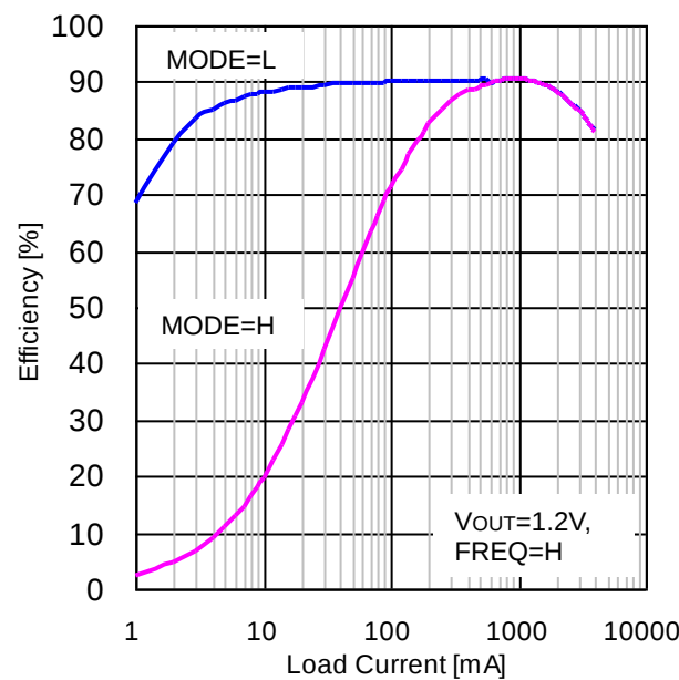
Figure 7. Efficiency vs Load Current (VIN=5V, VOUT=1.2V, L=1.0μH, FREQ=H)
