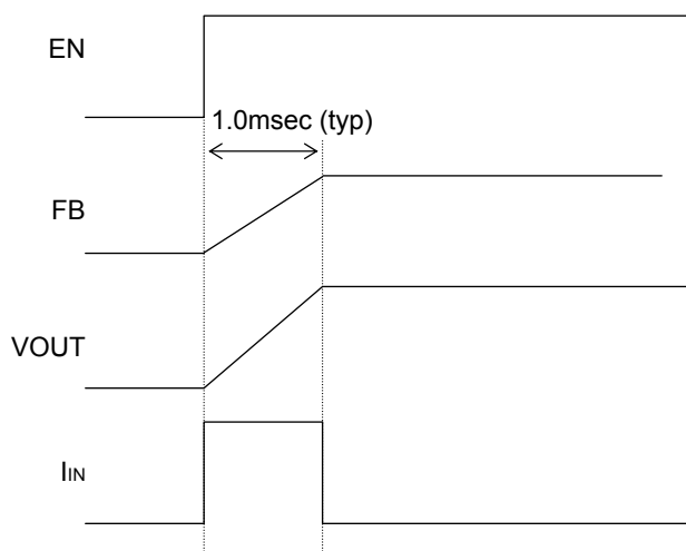
Figure 17. Soft Start Timing Chart
