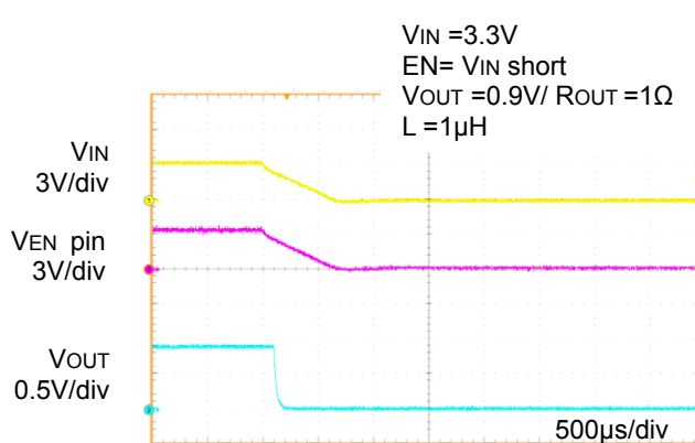
Figure 11. Shutdown (with V_{IN} UVLO)
