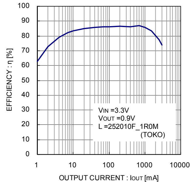
Figure 21. Efficiency
