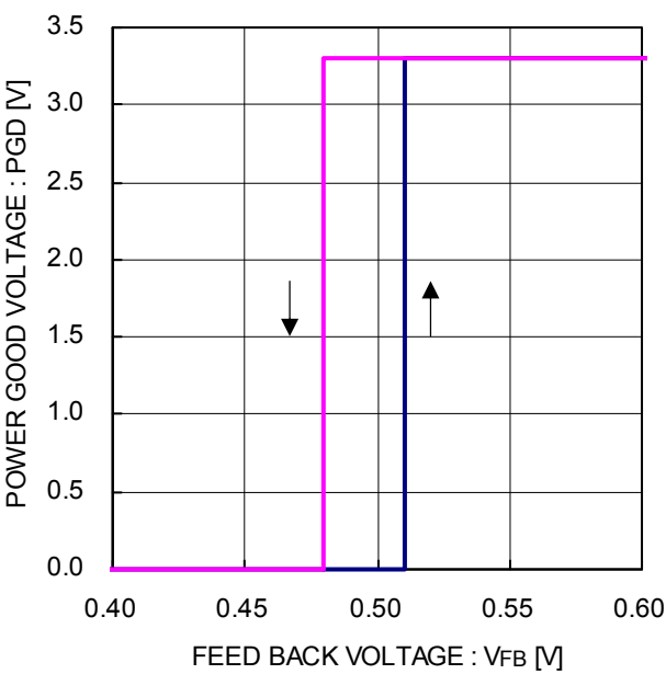
Figure 24. Power Good voltage/hysteresis
