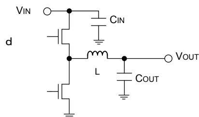
Figure 39. Input capacitor
