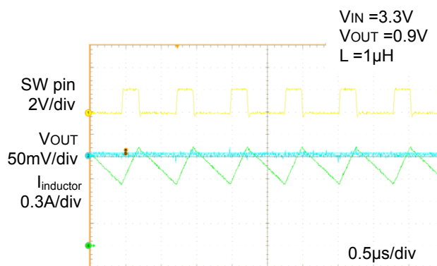
Figure 7. PWM operation, load 1000mA
