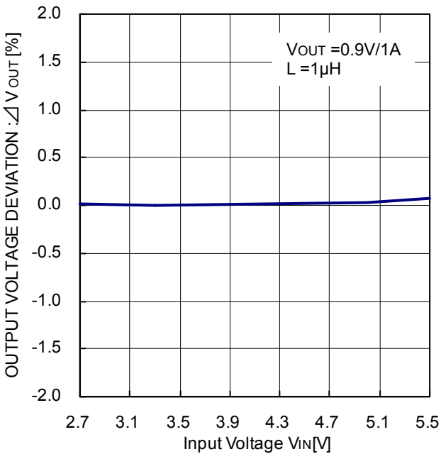
Figure 26. Output variation (Line regulation)
