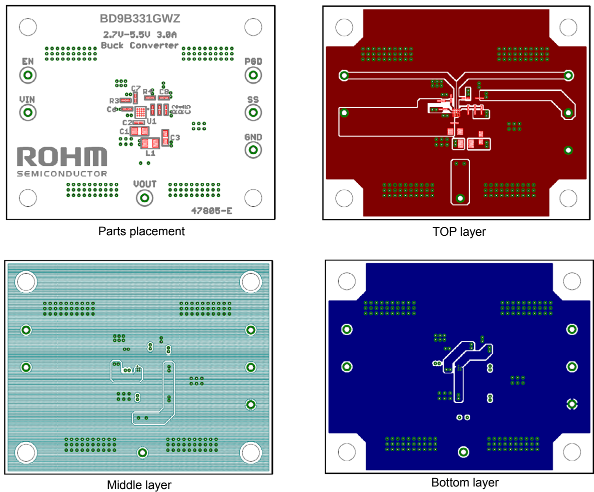
Figure 43. An example of PCB layout
