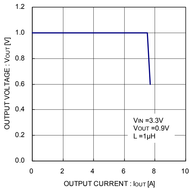
Figure 28. OCP detection current
