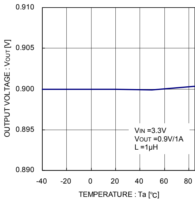
Figure 27. Output variation (ambient temperature)
