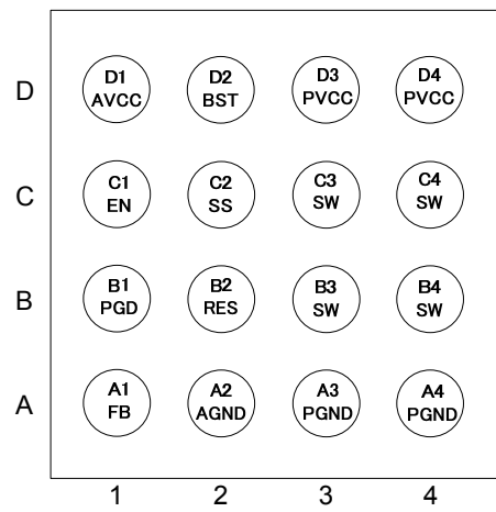
Figure 2. Pin Configuration
