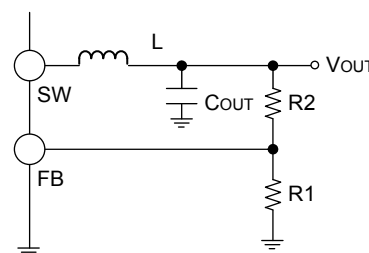
Figure 40. Output voltage setting resistor
