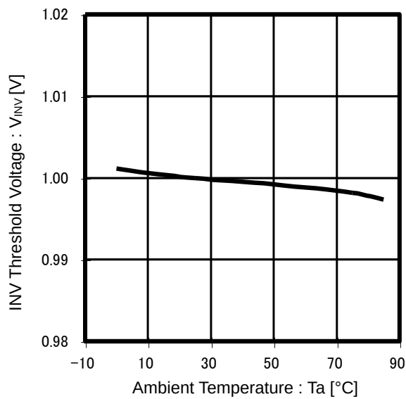
Figure 11. INV Threshold Voltage vs Ambient Temperature
