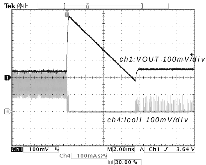
Figure 43. Io change PFM 100mA=>1mA VIN=2.4V
