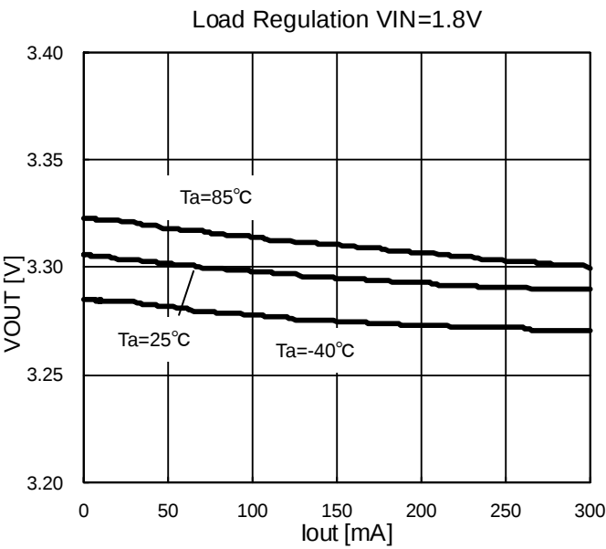
Figure 16. Load Regulation PWM VIN=1.8V
