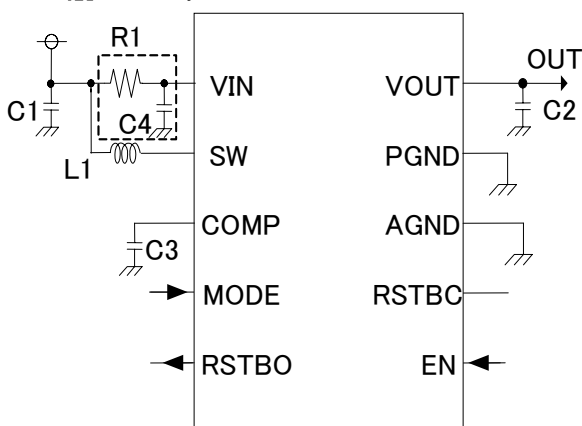
Figure 1. Application Circuit
