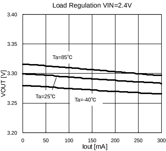
Figure 17. Load Regulation PWM VIN=2.4V
