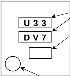
VSON010V3030 (TOP VIEW)
