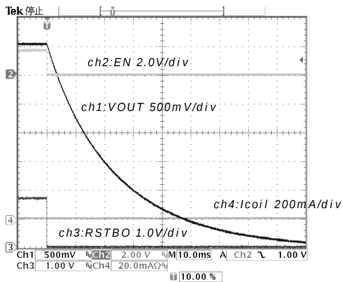
Figure 29. FALL [EN : ON=>OFF] PFM VIN=2.4V Io=0mA
