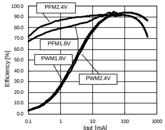
Figure 2. Efficiency
