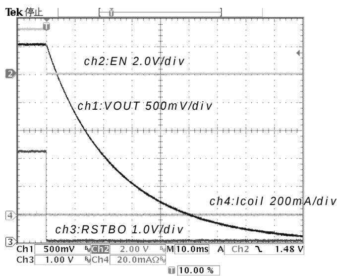
Figure 31. FALL [EN : ON=>OFF] PFM VIN=3.2V Io=0mA
