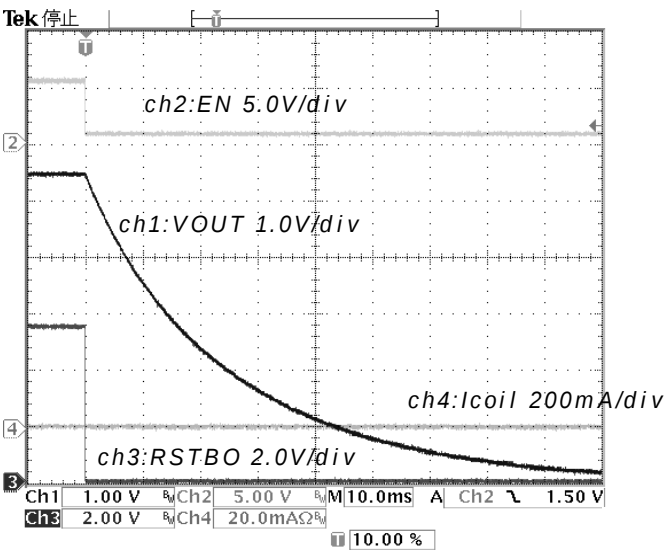
Figure 33. FALL [EN : ON=>OFF] PFM VIN=5.5V Io=0mA
