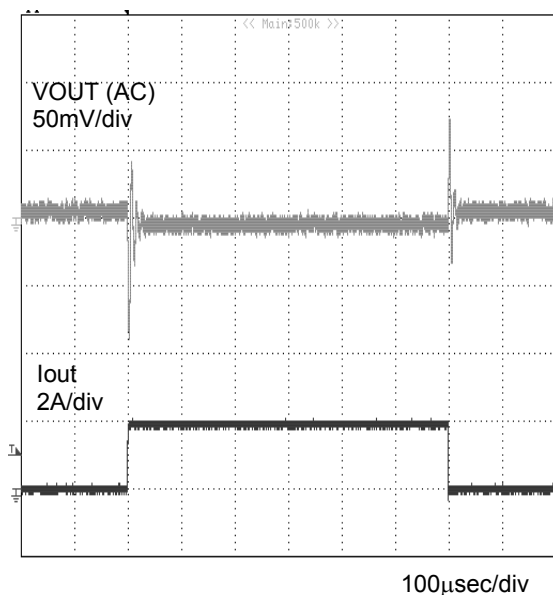
Figure 14. VOUT Transient Response ( V_{\text{IN}}=12\text{V} , V_{\text{OUT}}=3.3\text{V} , L=3.3\mu\text{H} , C_{\text{OUT}}=44\mu\text{F} , I_{\text{out}}=0\leftrightarrow 2\text{A} ( \text{SR}=1.0\text{A}/\mu\text{sec} ))
