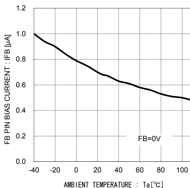
Figure 16. FB pin bias current vs. temperature characteristics
