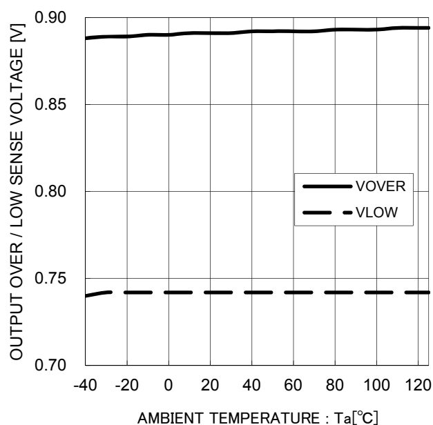
Figure 18. Output overvoltage / undervoltage detection voltage vs. temperature characteristics
