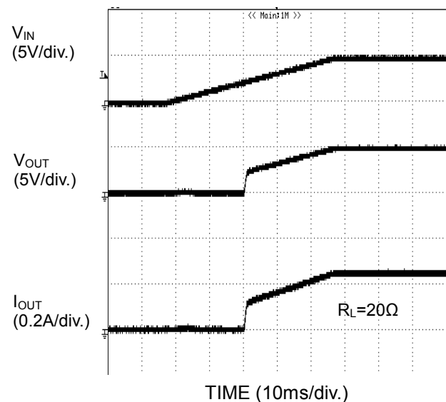
Figure 39. UVLO Response when Increasing V<sub>IN</sub>
