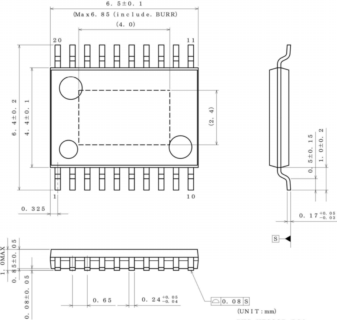
PKG : HTSSOP-B20 Drawing No. EX192-5002
