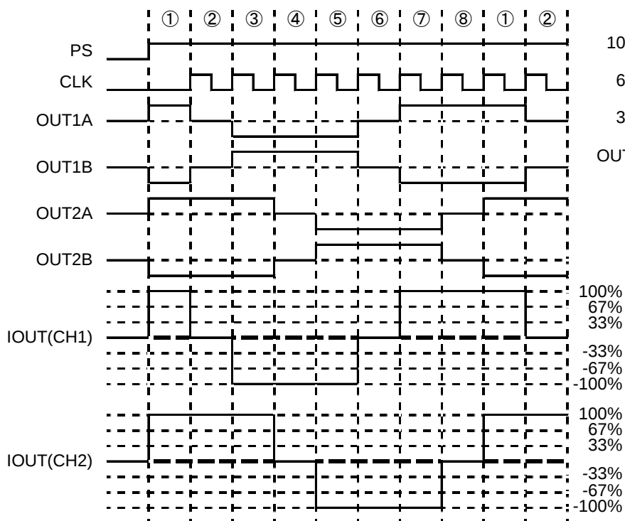
HALF STEP A (MODE0=H, MODE1=L, CW=L, ENABLE=H)
