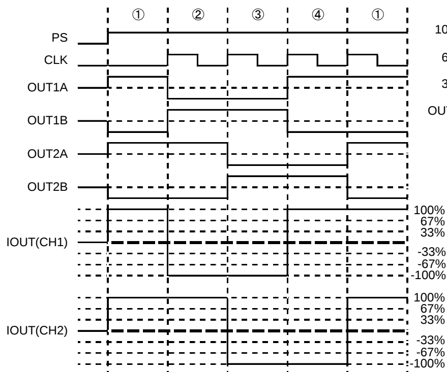
FULL STEP (MODE0=L, MODE1=L, CW=L, ENABLE=H)
