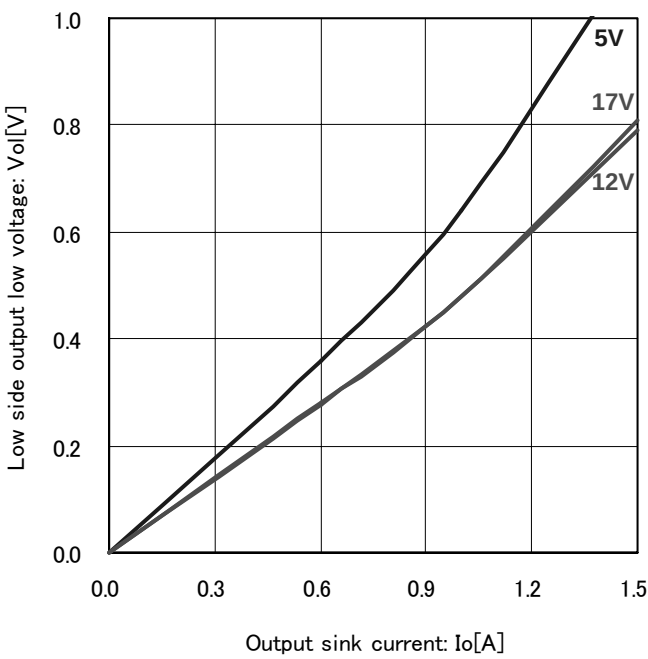
Fig.8 Low side output low voltage ( T_a=25^{\circ}C )
