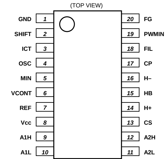
Fig.1 Pin configuration
