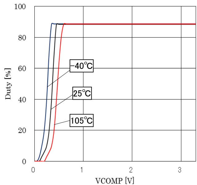
Figure 11. COMP V.S.DUTY
