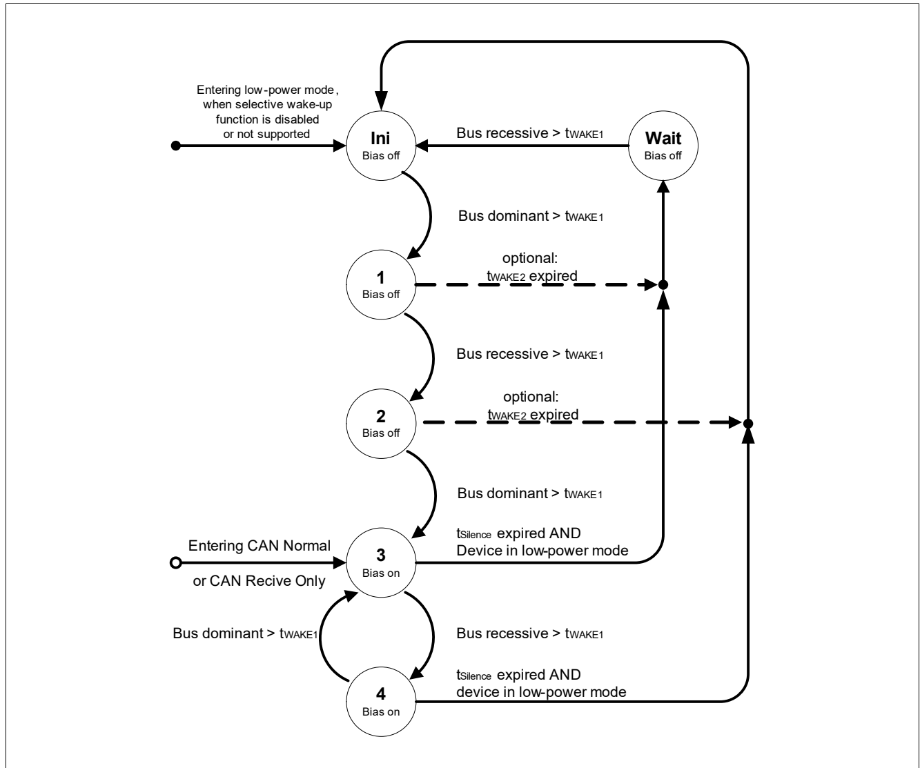
Figure 29 WUP detection following the definition in ISO 11898-2:2016
