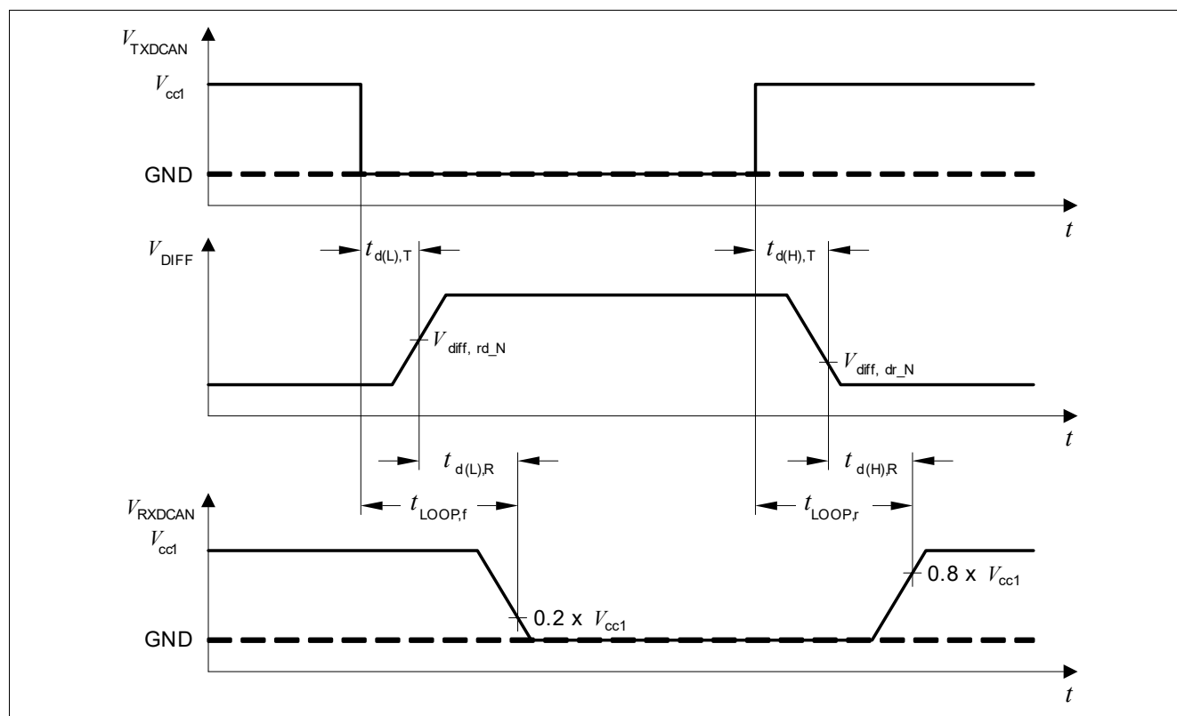
Figure 30 Timing Diagrams for Dynamic Characteristics
