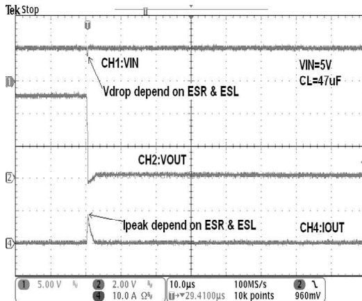
Inrush Short Circuit Response
