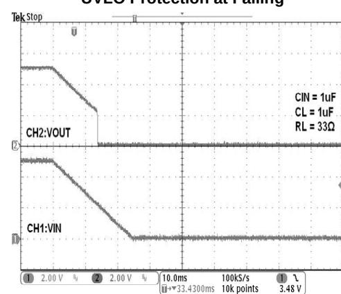
UVLO Protection at Falling
