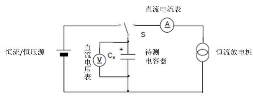
图1 恒流放电方法电路Constant current discharge method and circuit
