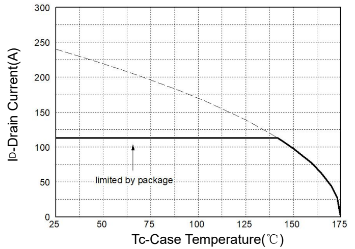
Figure 2: Drain Current
