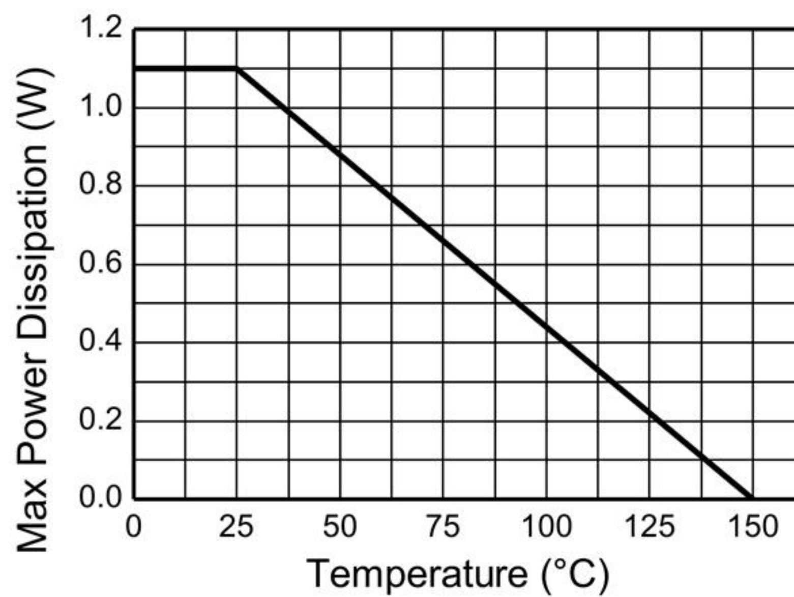
Derating Curve
