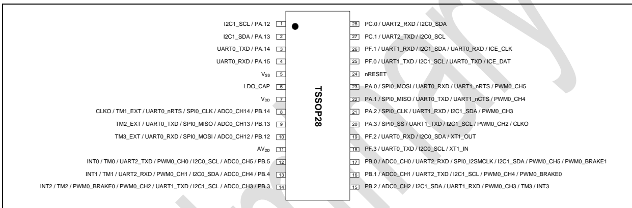
Figure 4.1-14 M031EC1AE Multi-function Pin Diagram
