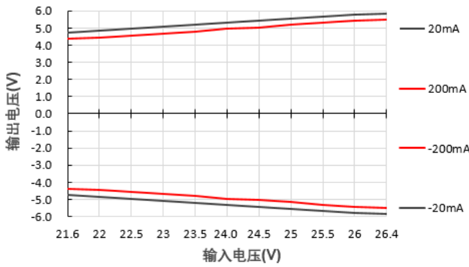
输出电压Vs输入电压@E2405S-2WR3
