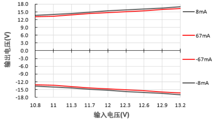
输出电压Vs输入电压@E1215S-2WR3
