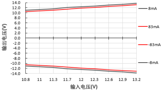
输出电压Vs输入电压@E1212S-2WR3
