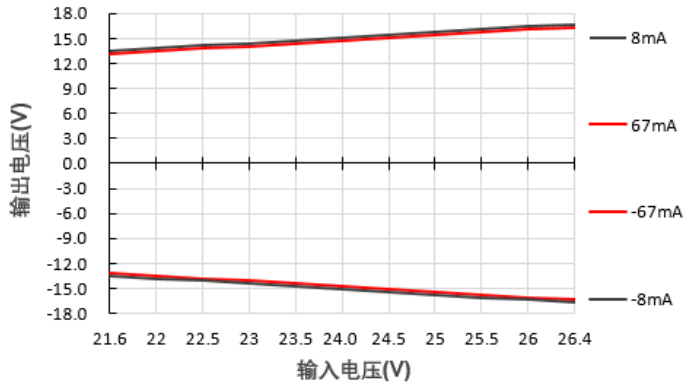
输出电压Vs输入电压@E2415S-2WR3
