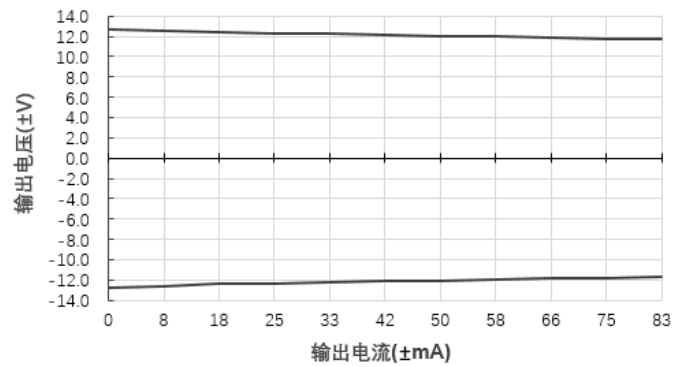
输出电压Vs输出电流(Vin=5V)@E0512S-2WR3
