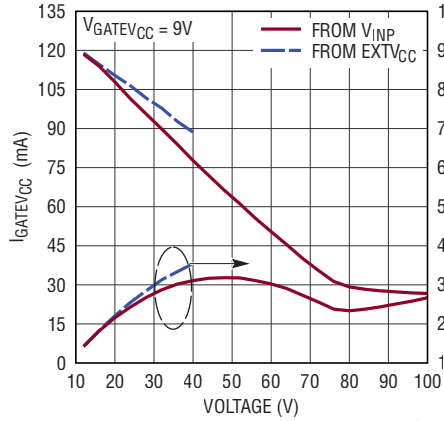
GATEV CC Max Current vs Voltage
