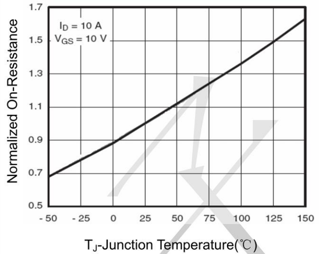
Figure 8 Drain-Source On-Resistance
