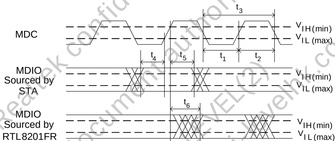
Figure 22. MDC/MDIO Timing
