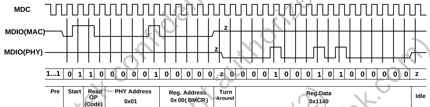
Figure 4. Read Cycle
