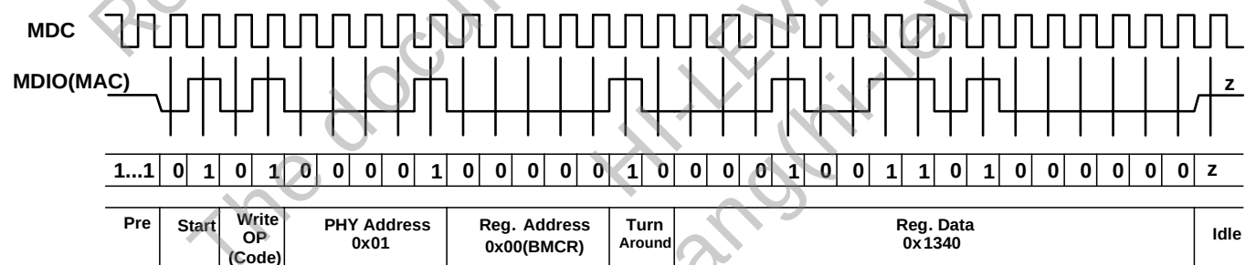
Figure 5. Write Cycle
