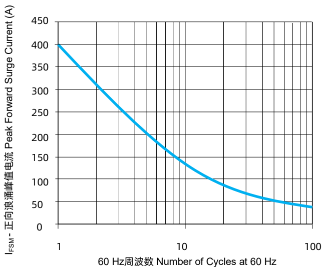
FIGURE 7 最大非重复正向浪涌电流(单向型) Maximum Non-Repitative Forward Surge Current Uni-Directional only
