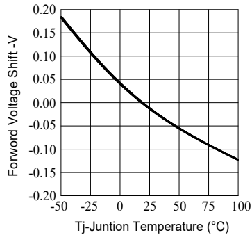
Fig.1-Forward Voltage Shift vs. Junction Temperature
