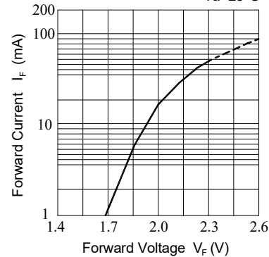
Fig.4-Forward Current vs. Forward Voltage T_a=25^{\circ}\text{C}
