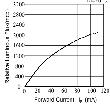
Fig.2-Relative Luminous Intensity vs. Forward Current T_a=25^{\circ}\text{C}
