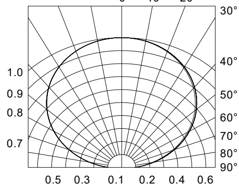
Fig.6-Radiation Diagram
