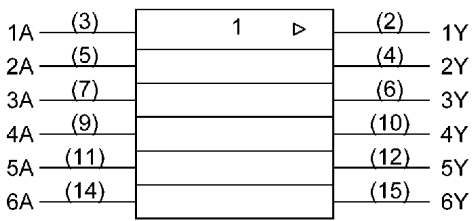
74HC4050D
