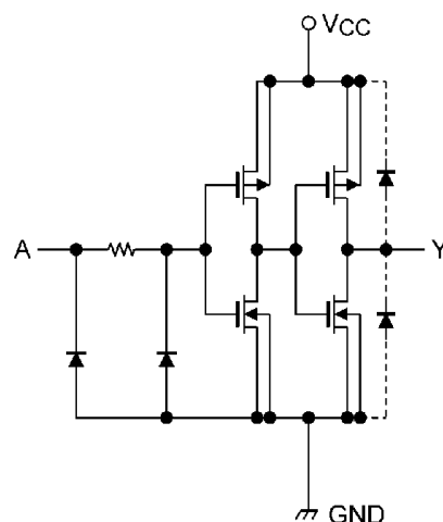
74HC4050D
