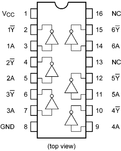
74HC4049D
