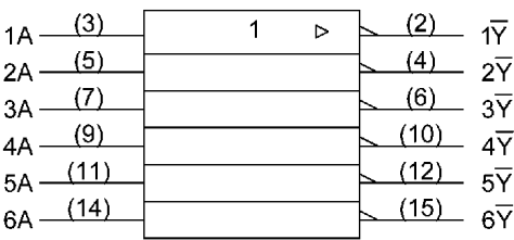
74HC4049D
