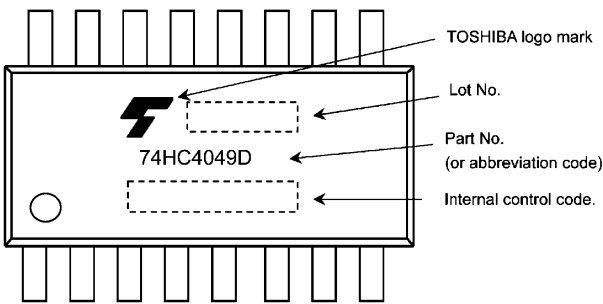
74HC4049D
