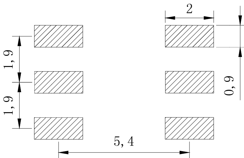
HP206F pad layout (unit: mm)
