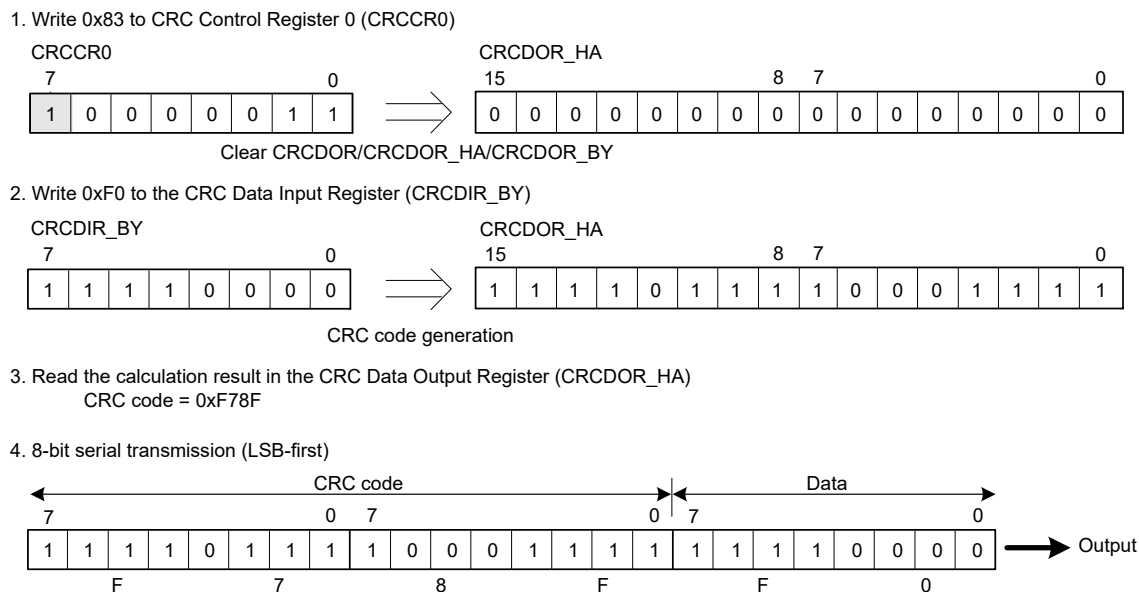
Figure 37.2 LSB-first data transmission
