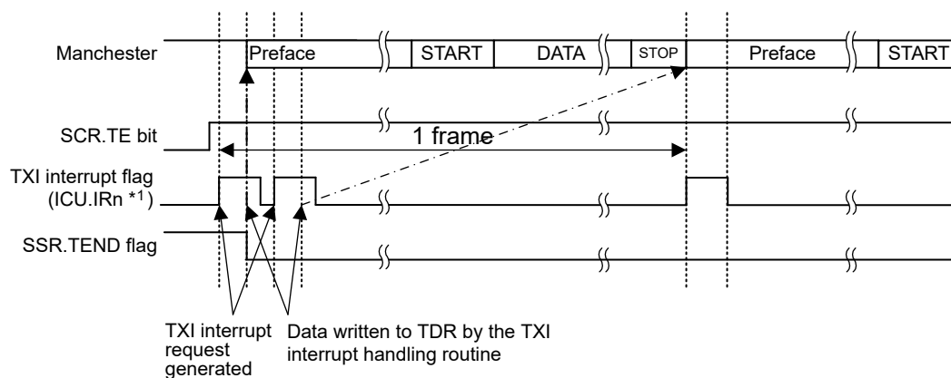
Figure 29.56 Example of Start-of-Transmission Operation for Serial Transmission in Manchester mode (with Preface but Without the CTS Function)
