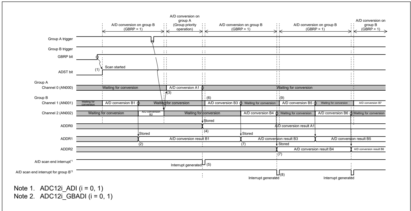
Figure 40.23 Group priority operation example 1-5: Continuously activating single scan for group B (when ADGSPCR.GBRP = 1, ADGSPCR.LGRRS = 0)
