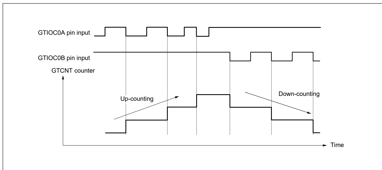
Figure 21.51 Example of phase counting mode 3 (A)
