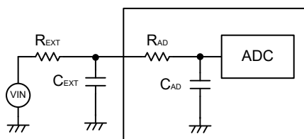
Figure 40.40 Sample and hold circuit simplified diagram
