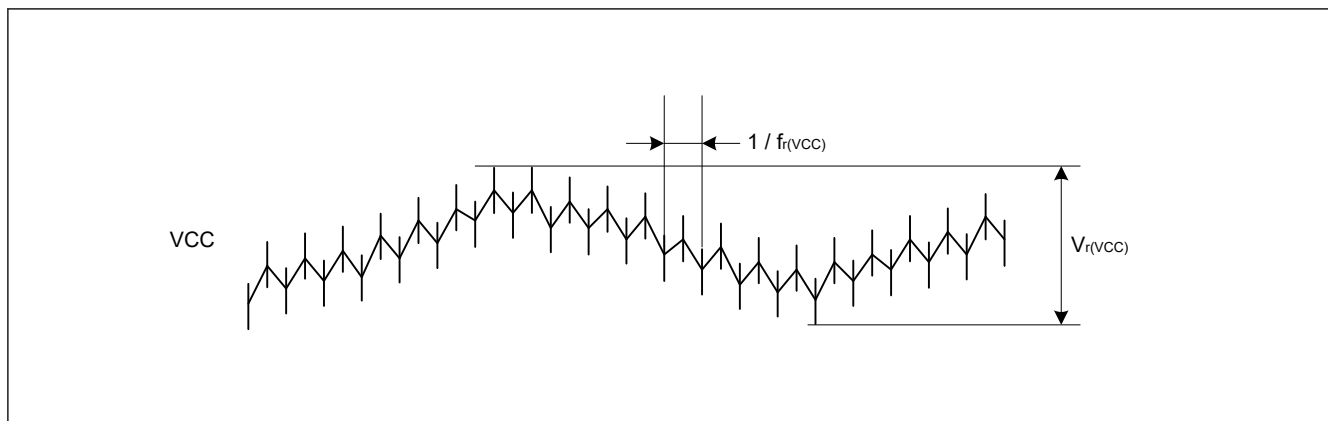
Figure 50.6 Ripple waveform
