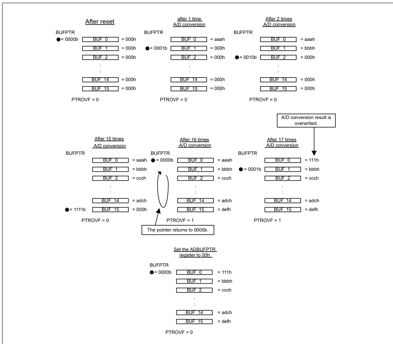
Figure 40.31 Data Buffers, Pointer, and Overflow Flag Operations
