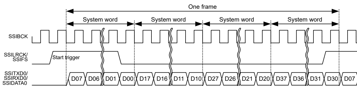
Figure 35.41 TDM format (without padding: system word length = data word length)
