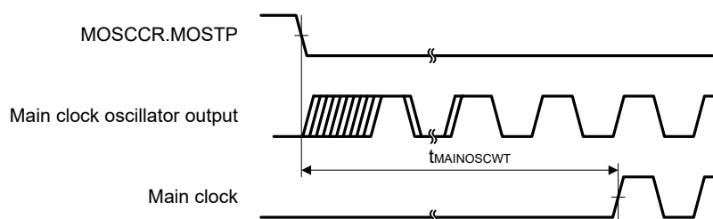
Figure 50.9 Main clock oscillation start timing
