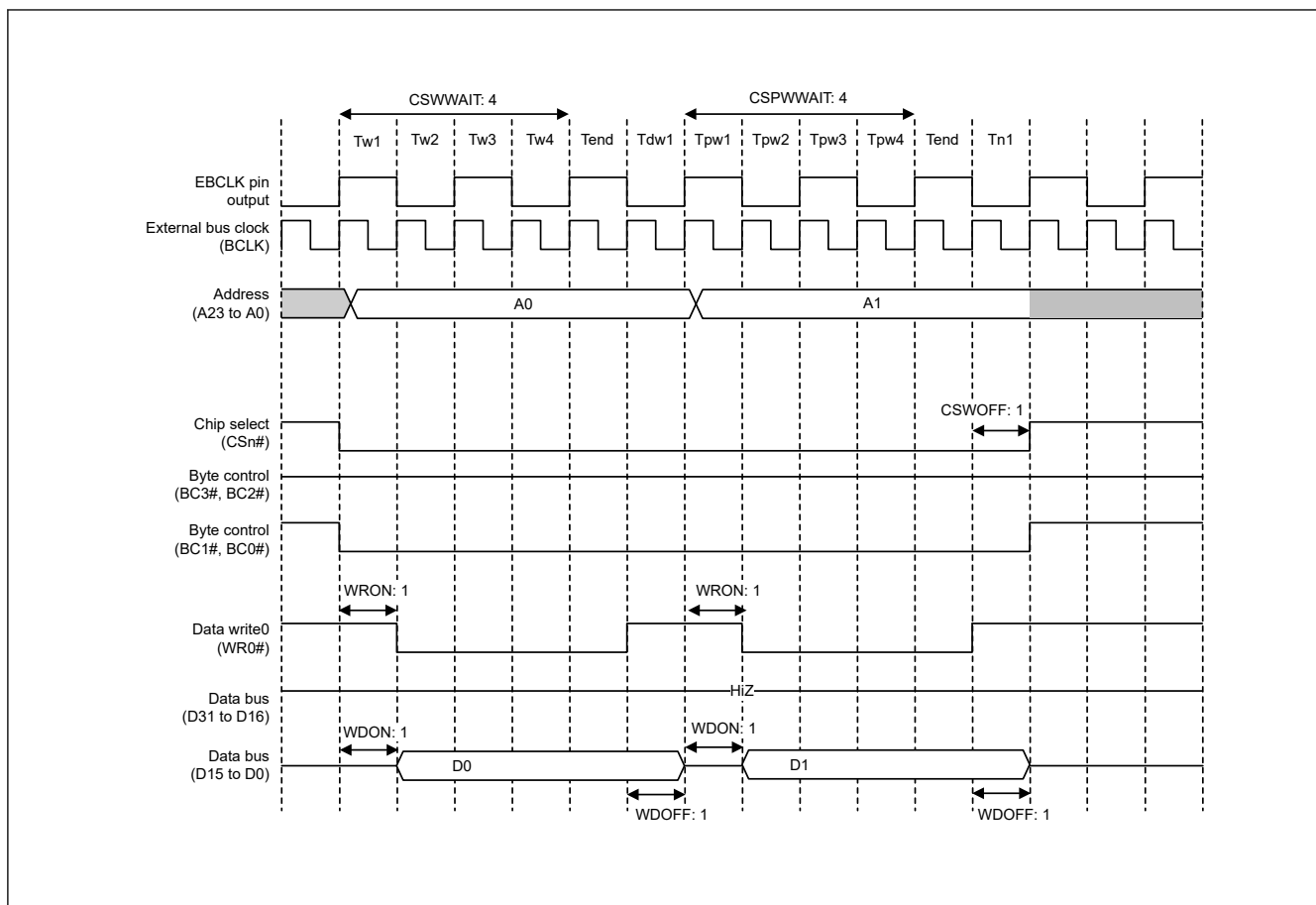
Figure 14.22 Example of page write access operation when BCLK/2 is selected in the EBCLK Pin Output Select Bit and two rounds of bus access are generated in response to a single transfer request in single-write strobe mode (n = 0 to 7)
