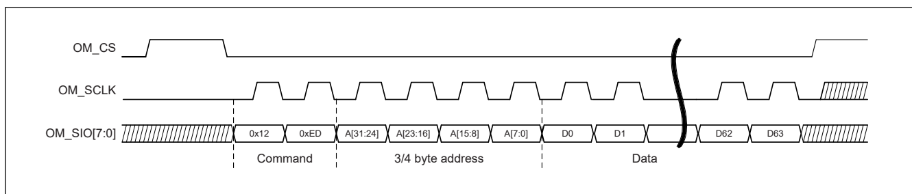
Figure 34.4 Waveform of Write Operation in OctaFlash interface (SOP Mode)
