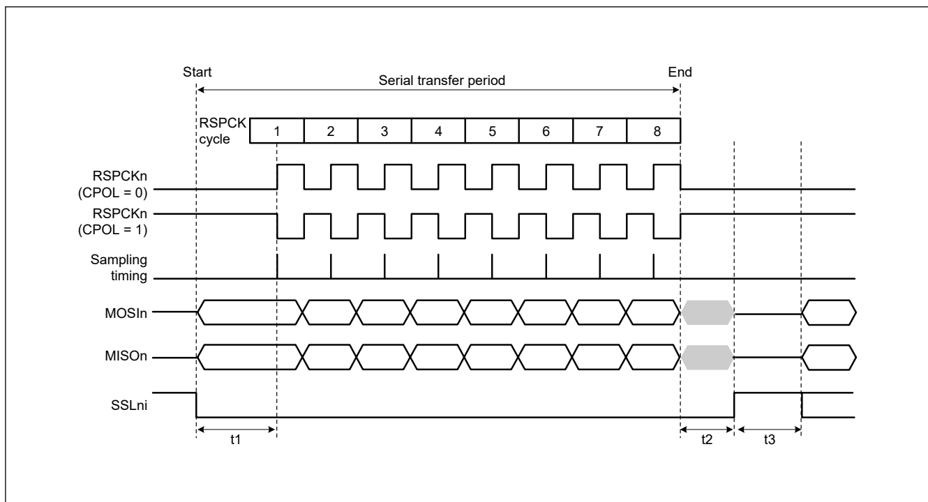
Figure 32.24 SPI transfer format when CPHA = 0
