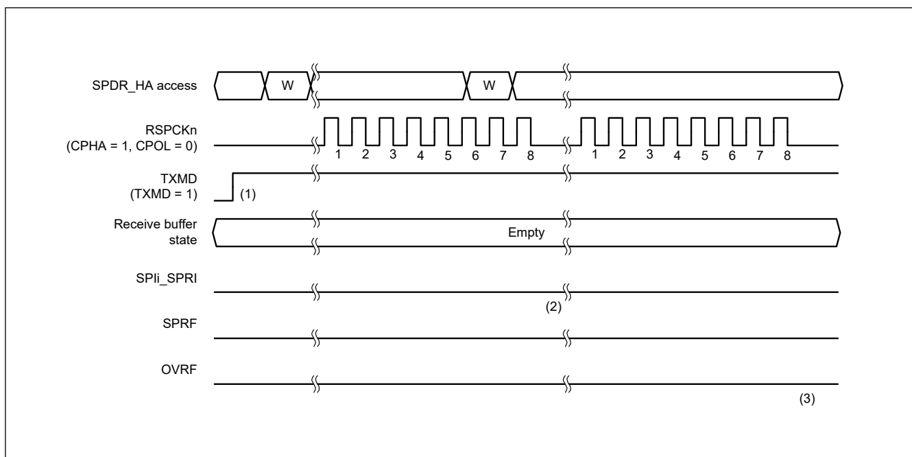
Figure 32.27 Operation example when SPCR3.ETXMD = 0 and SPCR.TXMD = 1
