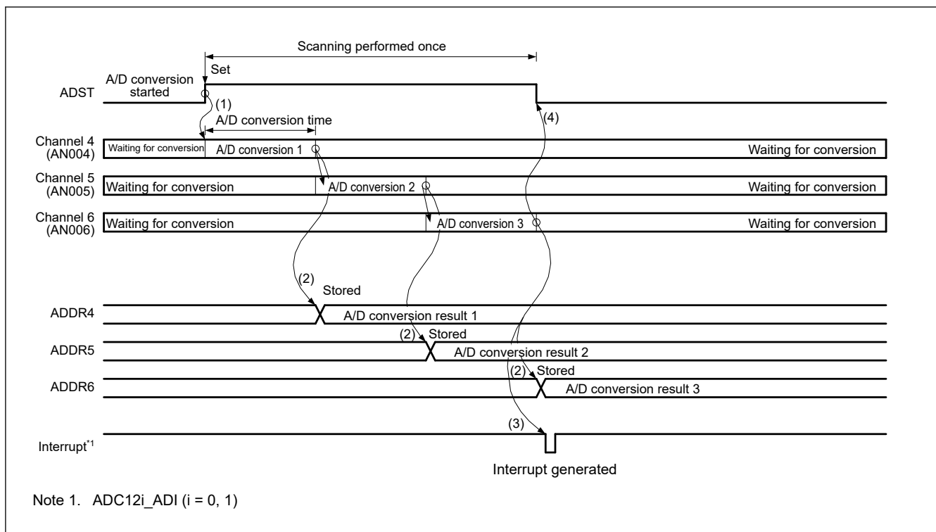
Figure 40.8 Example basic operation in single scan mode when AN004 to AN006 are selected
