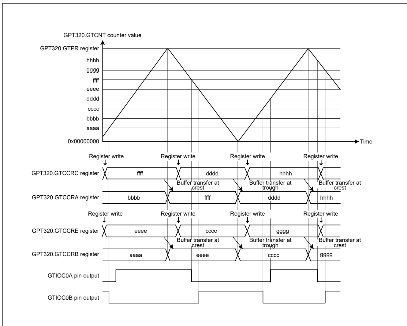
Figure 21.22 Example of triangle-wave PWM mode 2 operation with buffer operation, low output from the GTIOC0A pin and high output from the GTIOC0B pin at count start, output toggled at GTCCRA/GTCCRB compare match, and output retained at cycle end
