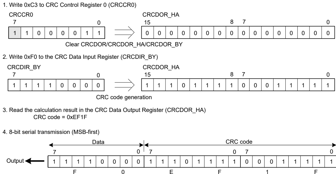
Figure 37.3 MSB-first data transmission
