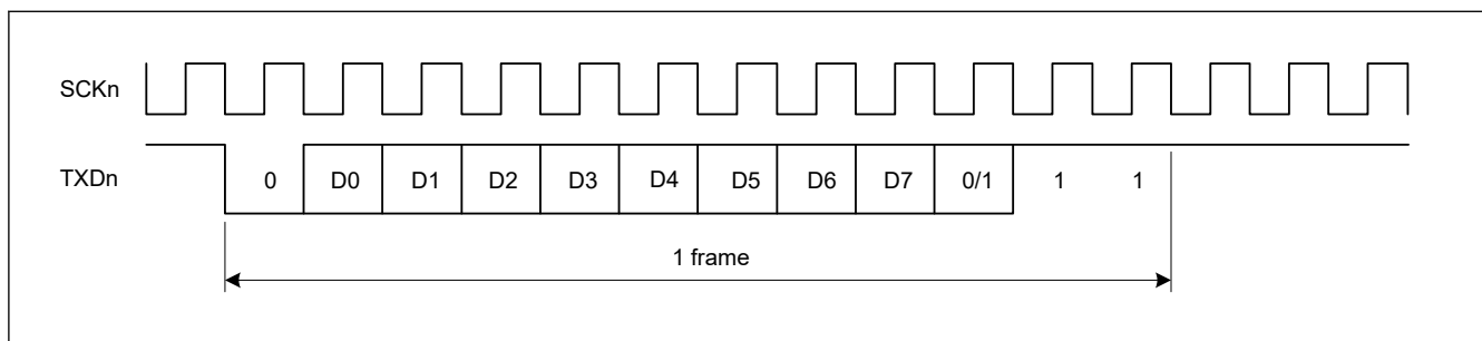
Figure 29.8 Phase relationship between output clock and transmit data in asynchronous mode when SMR.CHR = 0, PE = 1, MP = 0, and STOP = 1
