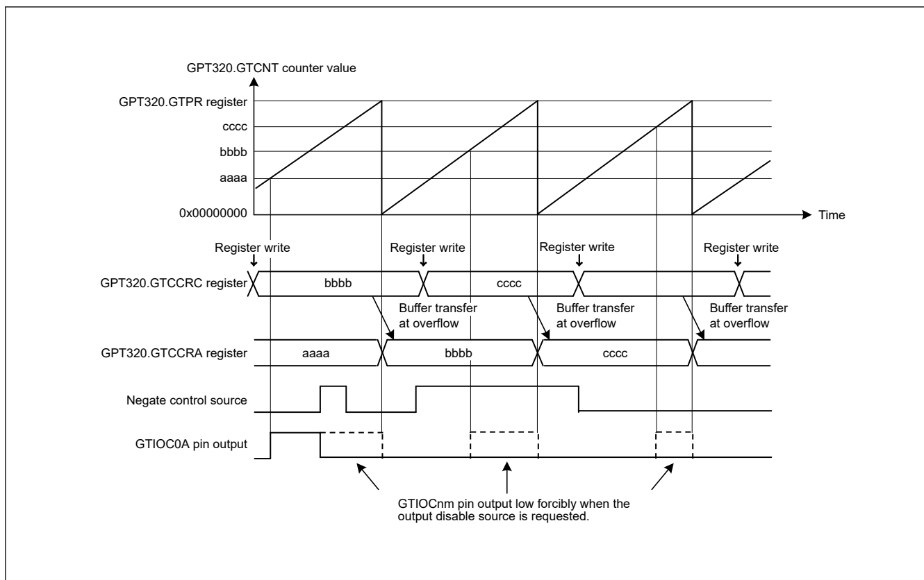
Figure 21.66 Example of GTIOCnm pin output disable control operation in saw-wave up-counting, buffer operation, active level 1, high output at GTCCRA compare match, low output at cycle end, and low output at output disable ( n = 0 to 9 , m = A, B )
