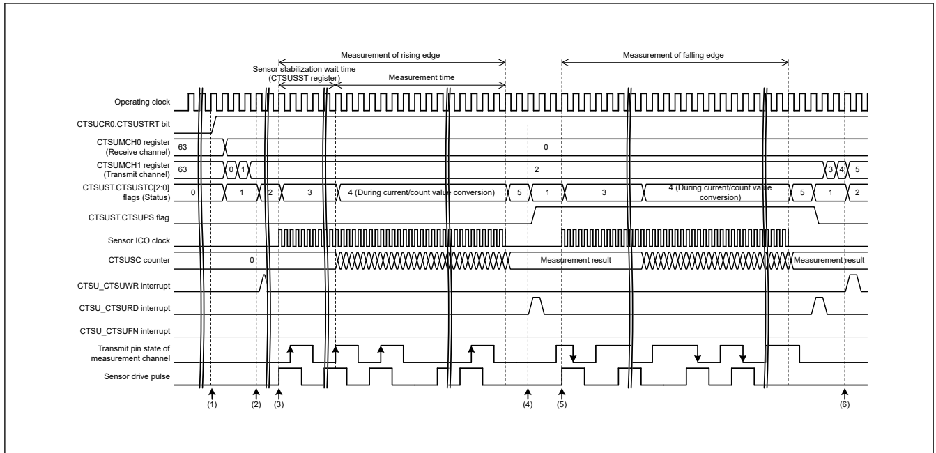
Figure 43.17 Timing of mutual capacitance full scan mode when the measurement start condition is a software trigger
