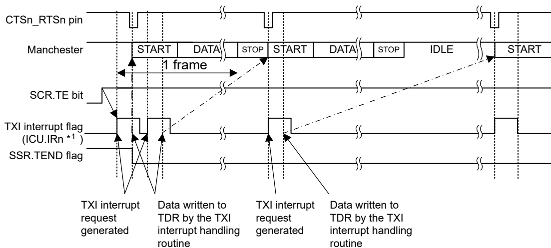
Figure 29.57 Example of Start-of-Transmission Operation for Serial Transmission in Manchester Mode (Without Preface but with the CTS Function)
