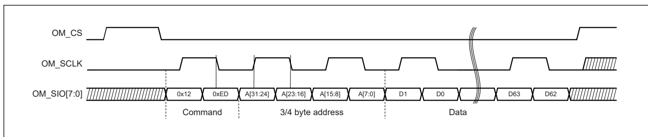
Figure 34.5 Waveform of Write Operation in OctaFlash interface (DOP Mode)
