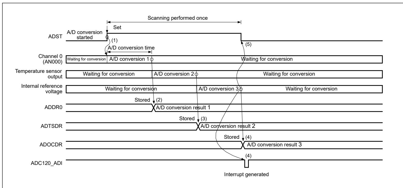
Figure 40.10 Example basic operation in single scan mode when AN000 and temperature sensor output or internal reference voltage are selected
