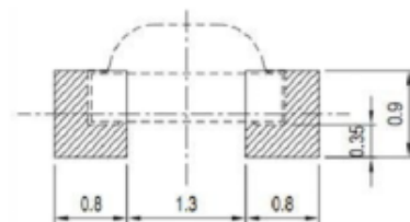
Soldering PAD Suggested:
