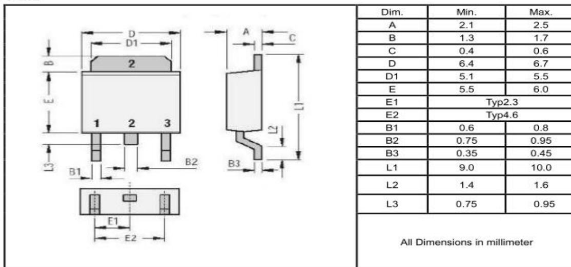
TO-252
