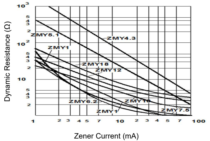
Fig 4. Dynamic Resistance vs.Zener Current
