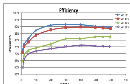
Efficiency @ Vout=5V
