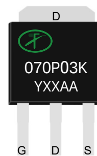
TO-251
