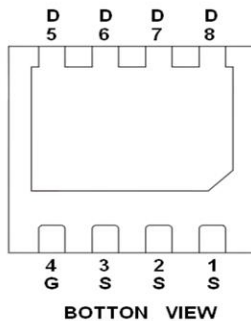
DFN3X3-8L
