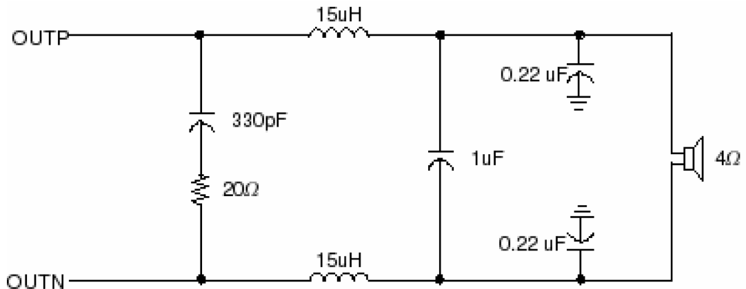
Figure 56. Typical LC filter for an 8 Ω speaker
