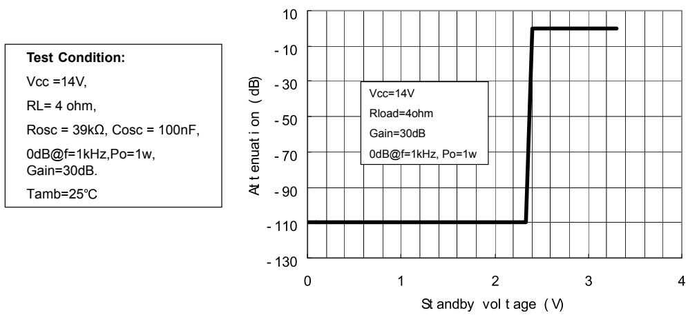
Figure 18. Attenuation vs. voltage on pin STBY
