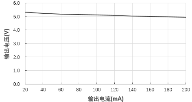
输出电压Vs输出电流(Vin=24V)@B2405LS-1WR3
