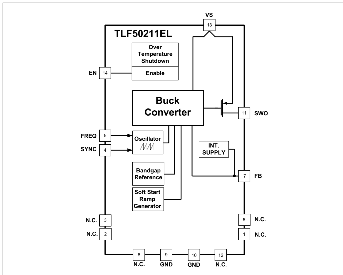
Figure 1 Block diagram
