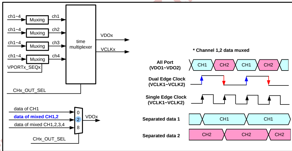
Figure 2.14 Block Diagram of Multiplexed 2-Channels Output
