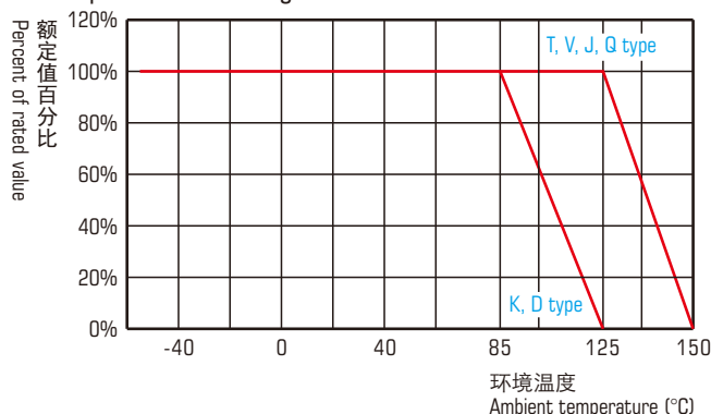
Temperature derating curves
