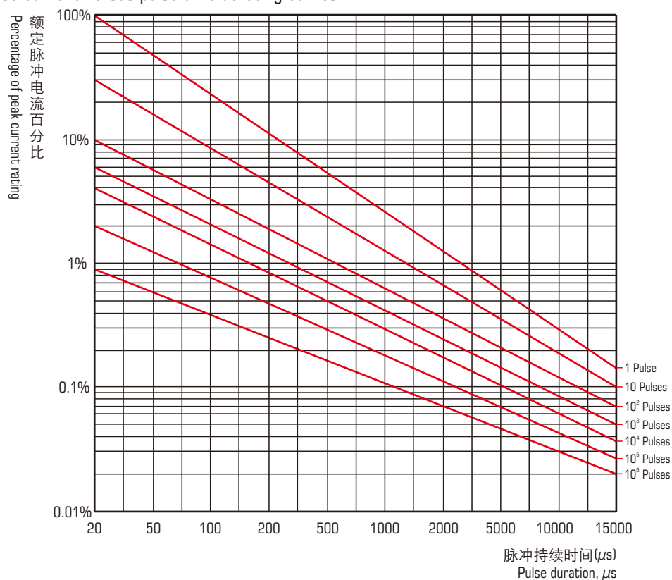
Pulse current versus pulse time derating curves
