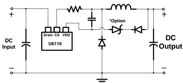
Buck Converter
