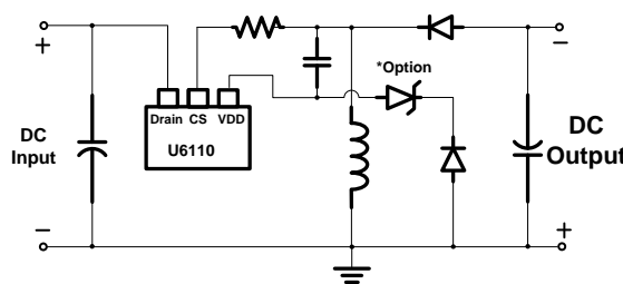
Buck/Boost Converter
