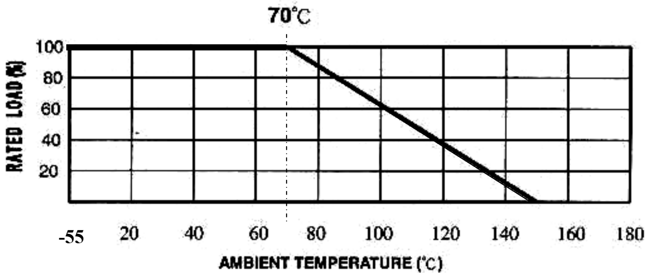
FIG.1 DERATING CURVE
